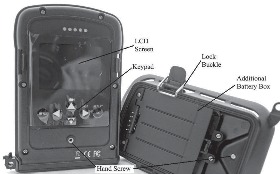
Figure 1.3: Back View of Ltl-5310M and Front View of Battery Box
