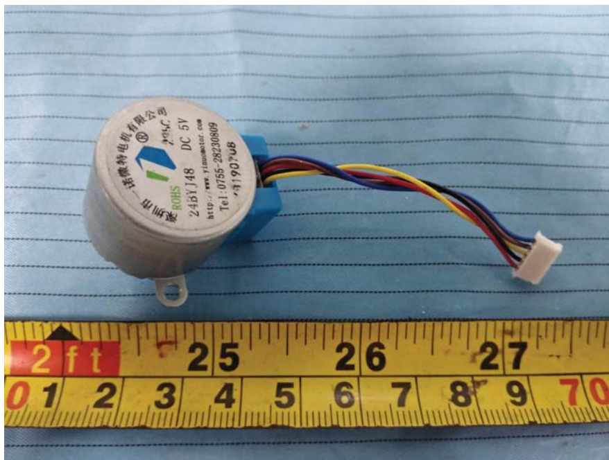
EUT – Motor 1 Top View
