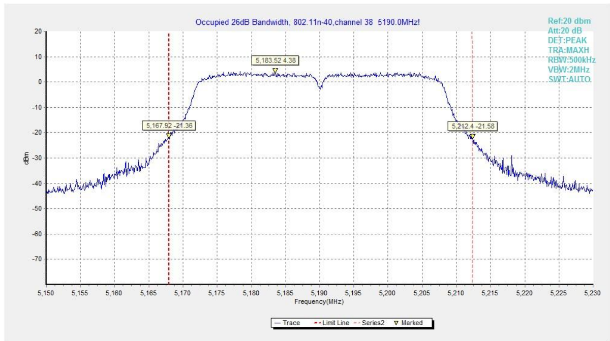
Fig. 19 Occupied 26dB Bandwidth (802.11n40, 5190MHz)
