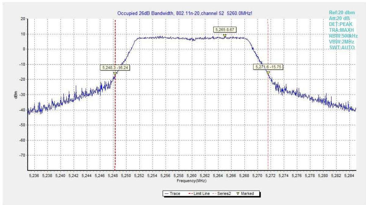
Fig. 13 Occupied 26dB Bandwidth (802.11n20, 5260MHz)
