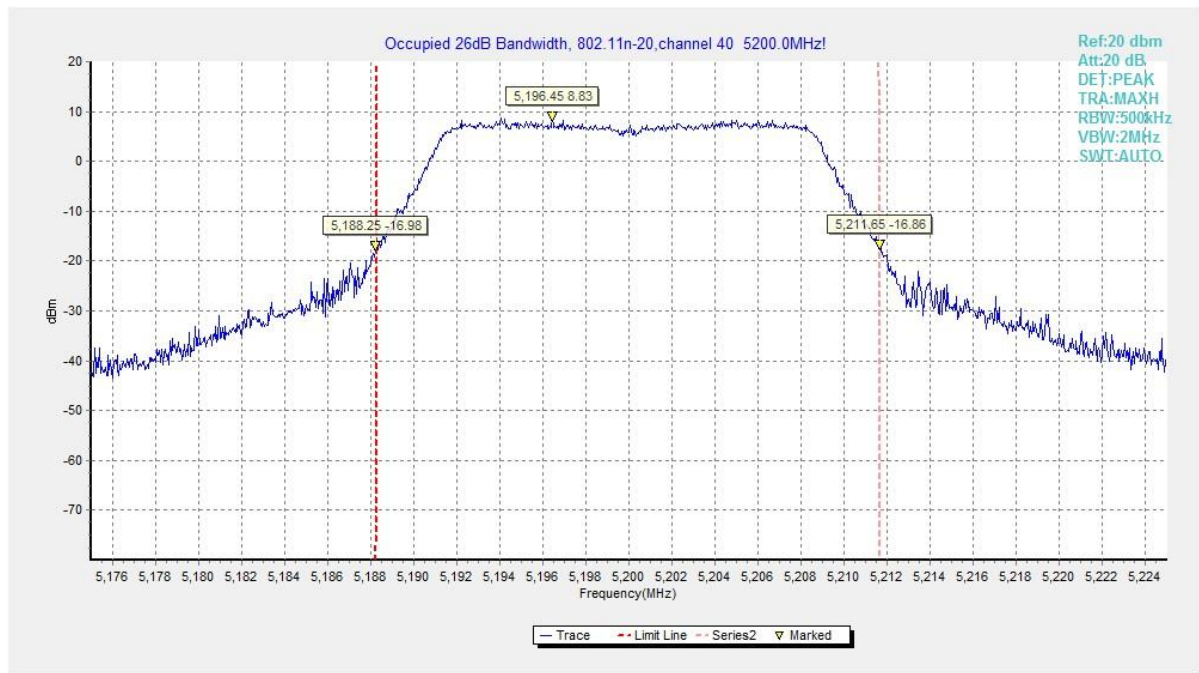
Fig. 11 Occupied 26dB Bandwidth (802.11n20, 5200MHz)
