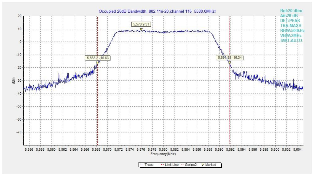
Fig. 17 Occupied 26dB Bandwidth (802.11n20, 5580MHz)
