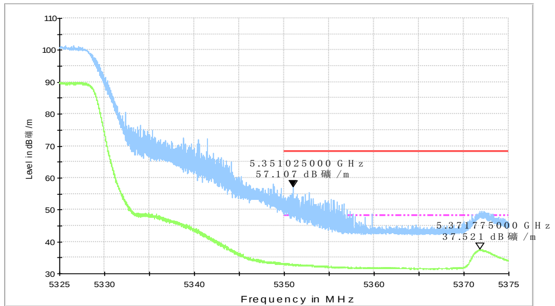
Fig. 31 Band Edges (802.11n-HT20, 5320MHz)
