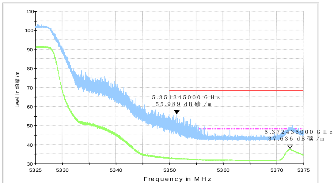
RE - Power-5.325GHz-5.375GHz
