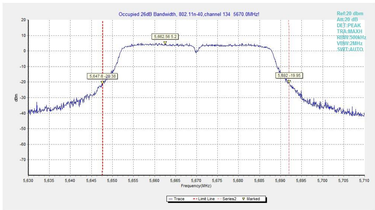
Fig. 25 Occupied 26dB Bandwidth (802.11n40, 5670MHz)
