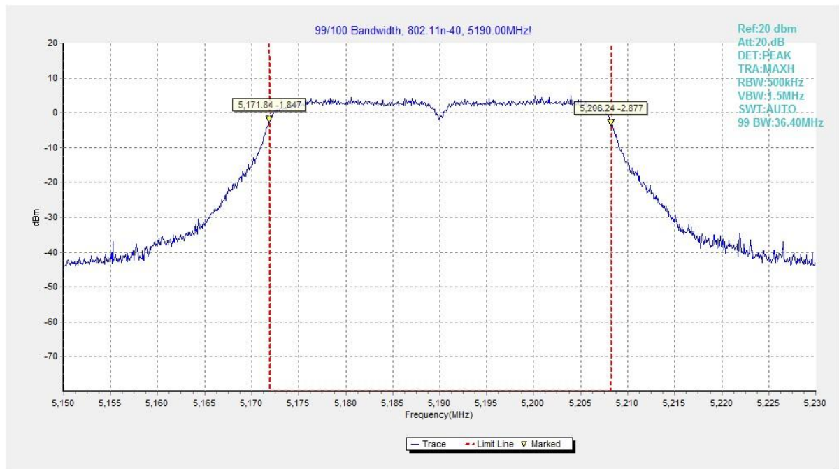
Fig. 47 99% Occupied bandwidth (802.11n40, 5190MHz)
