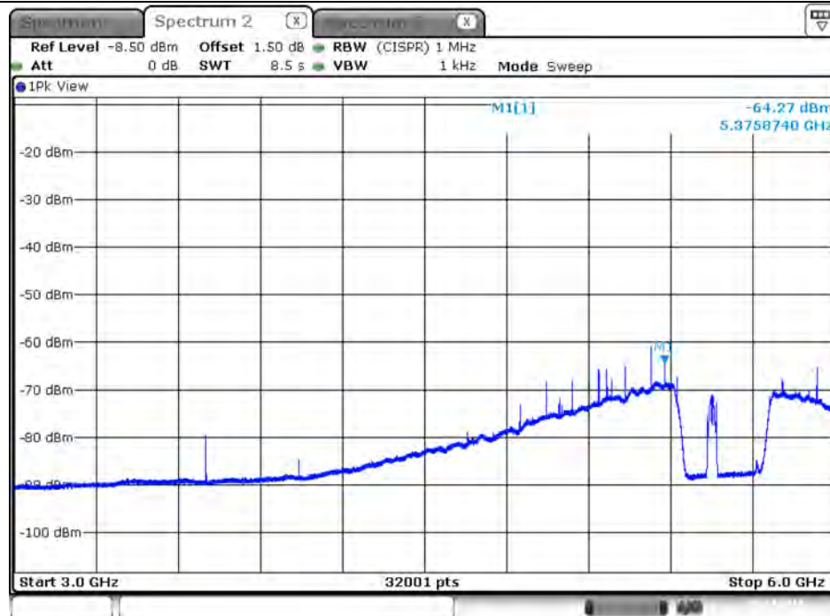
Plot on Configuration VHT40 / 5550 MHz / Average / Port 1 / 3GHz~6GHz
