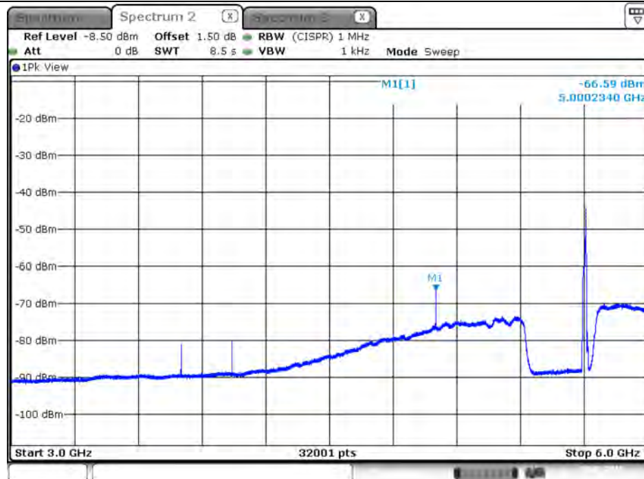
Plot on Configuration VHT20 / 5700 MHz / Average / Port 3 / 3GHz~6GHz
