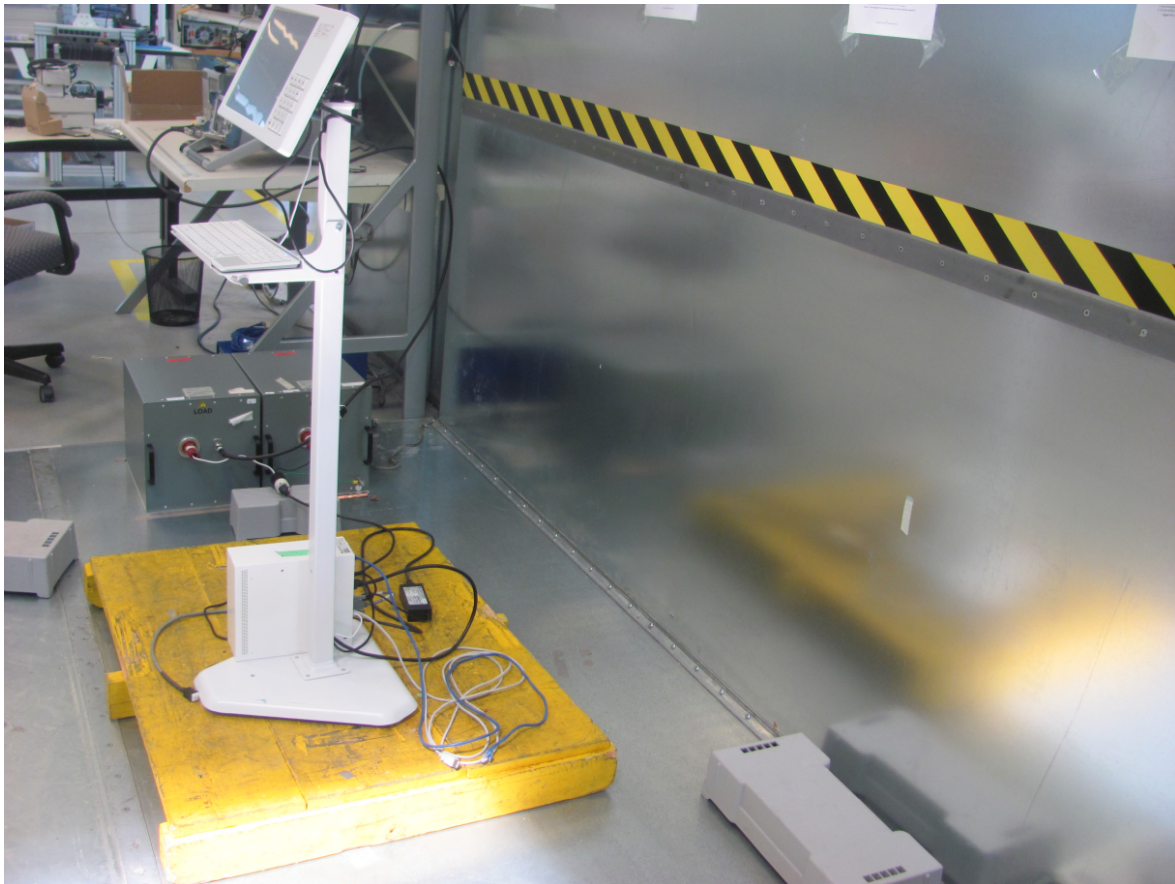
Figure 5 – Conducted Emissions Setup – Photo 2
