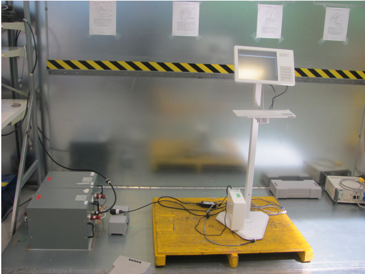
Figure 4 – Conducted Emissions Setup – Photo 1
