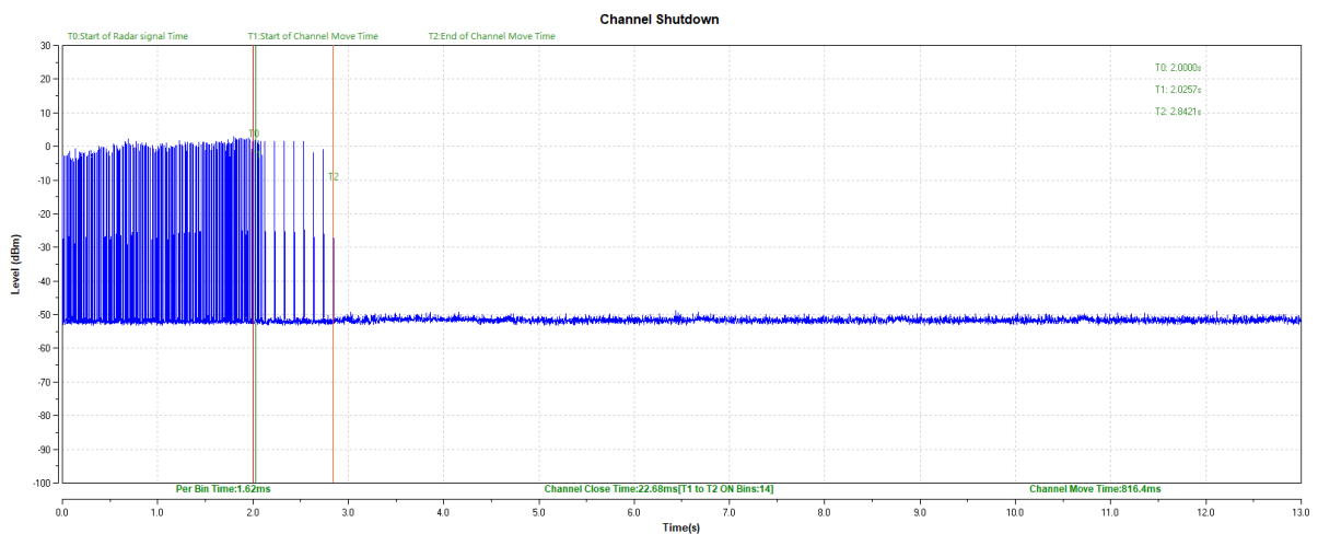
Fig.2 Channel Shutdown (HT80 Frequency Band: 5470MHz~5725MHz)
