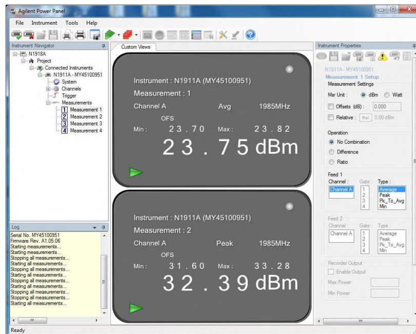
Uplink: LTE Band 25 20MHz BW High Ch & LTE Band 5 15MHz BW Low Ch
