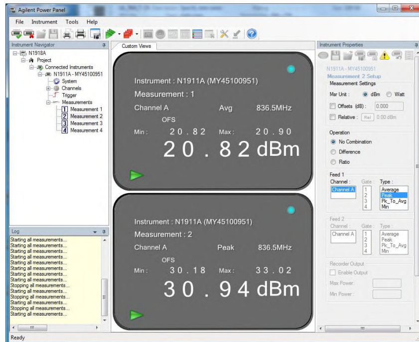
LTE Band 5_Uplink_5MHz Bandwidth_Mid Channel
