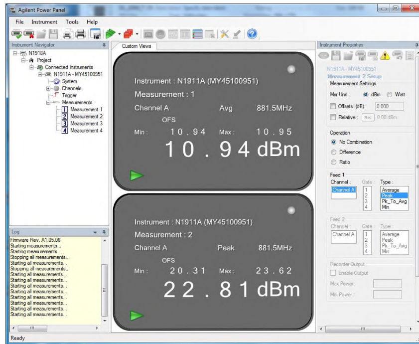
LTE Band 5_Downlink_5MHz Bandwidth_Mid Channel
