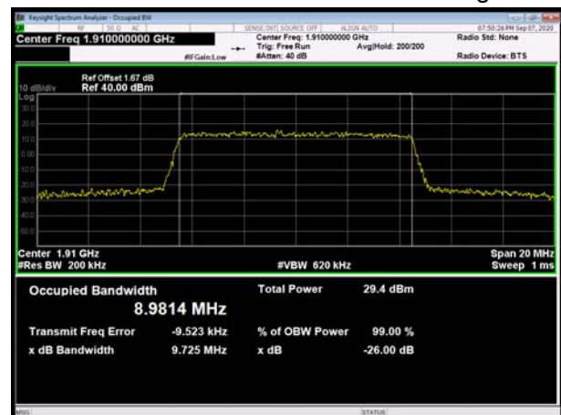
LTE Band 25 10MHz 16QAM CH-High
