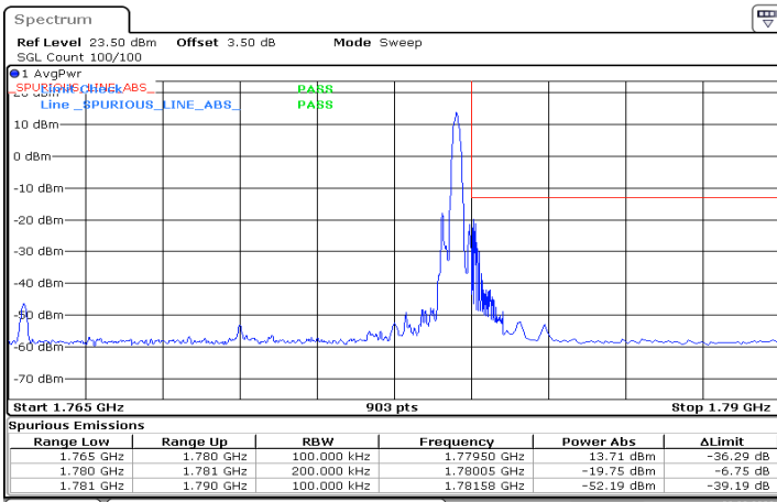
DC_12A_n66A_10MHz|15MHz_15kHz_707.5MHz|1772.5MHz_ DFT-s-OFDM QPSK_RB0|RB1@78
