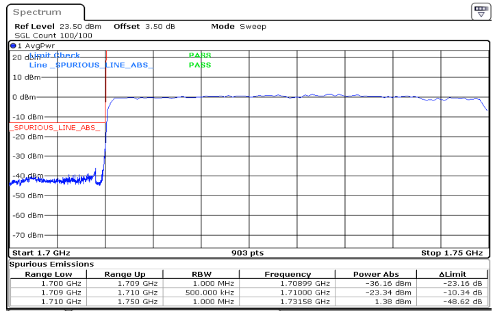
DC_12A_n66A_10MHz|40MHz_15kHz_707.5MHz|1730MHz_ DFT-s-OFDM QPSK_RB0|RB216@0
