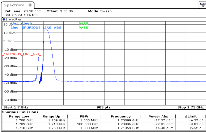
DC_12A_n66A_10MHz|40MHz_15kHz_707.5MHz|1730MHz_ DFT-s-OFDM QPSK_RB0|RB1@0
