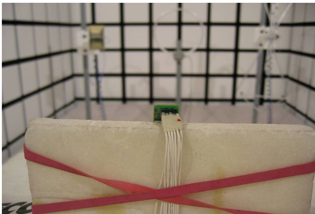
Photo 8: Measurements > 1GHz
