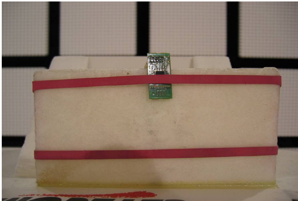
Photo 7: Measurements > 1GHz
