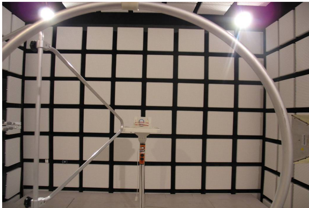
Photo 5: Measurements > 1GHz
