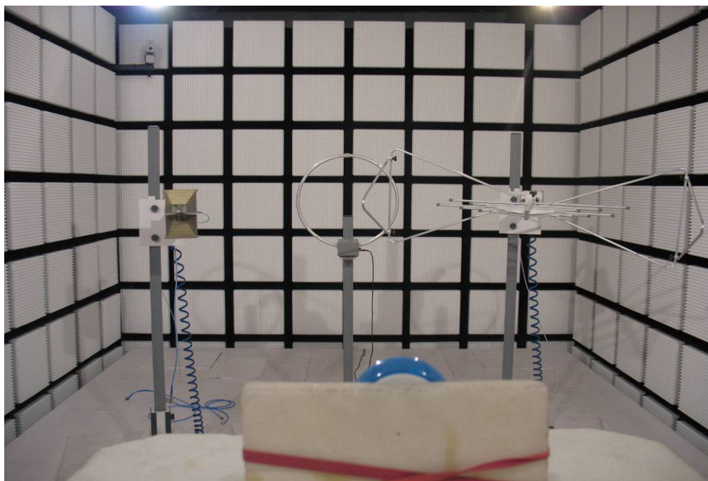
Photo 4: Measurements > 1GHz
