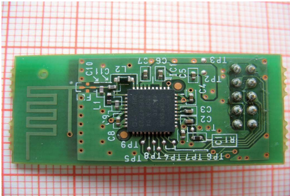
Photo 9: Module for radiated measurements
