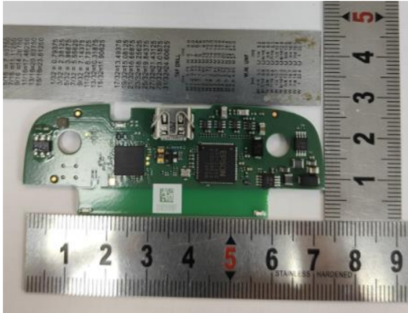
Main PCBA Top side view_ size: 73.6mm (length)*27.24mm (width)
