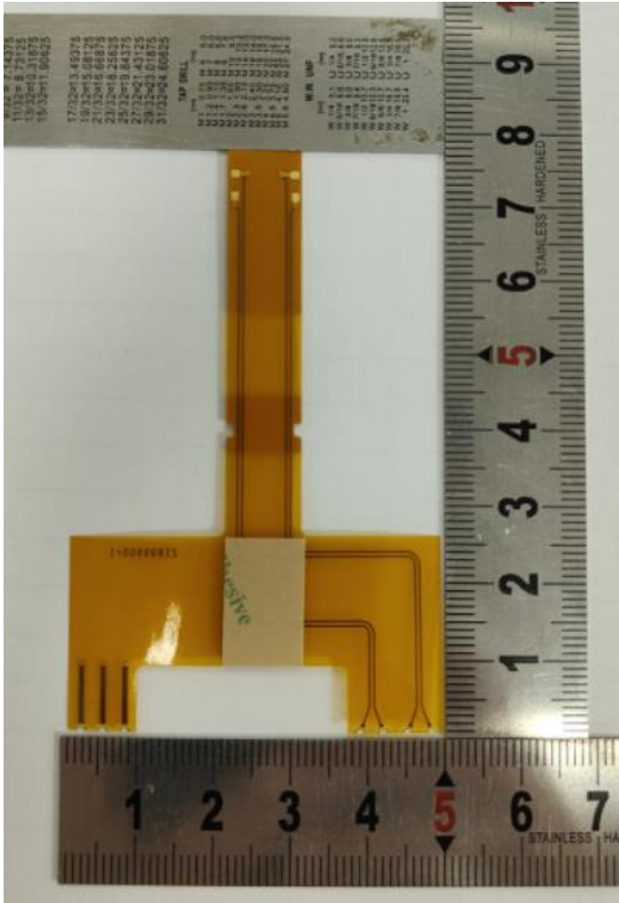
FPCBA Front side view_ size: 48.9mm (width)*76.73mm (height)
