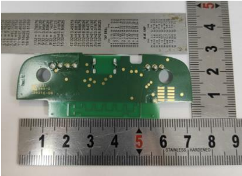
Main PCBA Bottom side view_ size: 73.6mm (length)*27.24mm (width)
