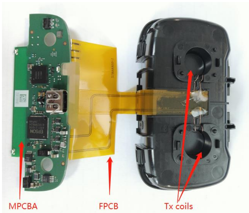
Internal configuration
