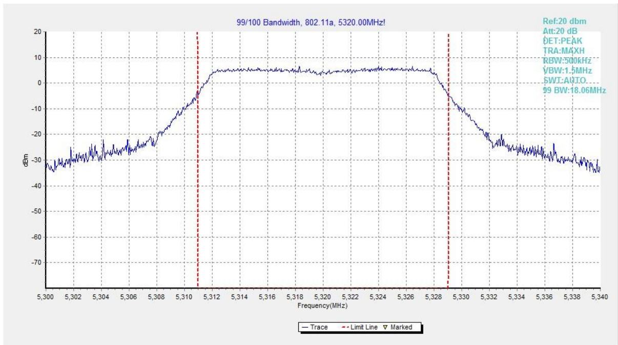
Fig. 27 99% Occupied Bandwidth (802.11a, 5320MHz)
