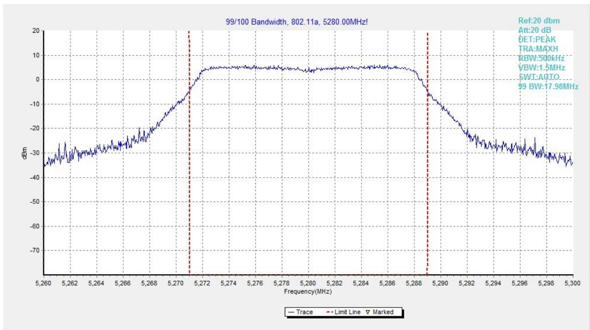
Fig. 26 99% Occupied Bandwidth (802.11a, 5280MHz)
