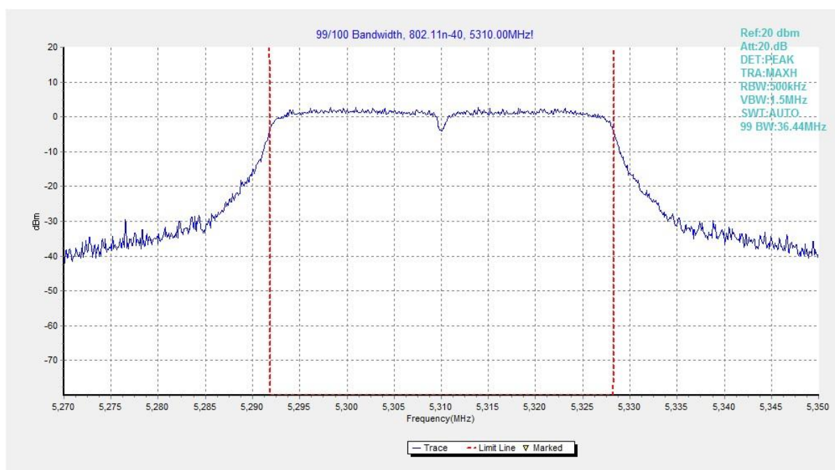
Fig. 34 99% Occupied Bandwidth (802.11n-HT40, 5310MHz)
