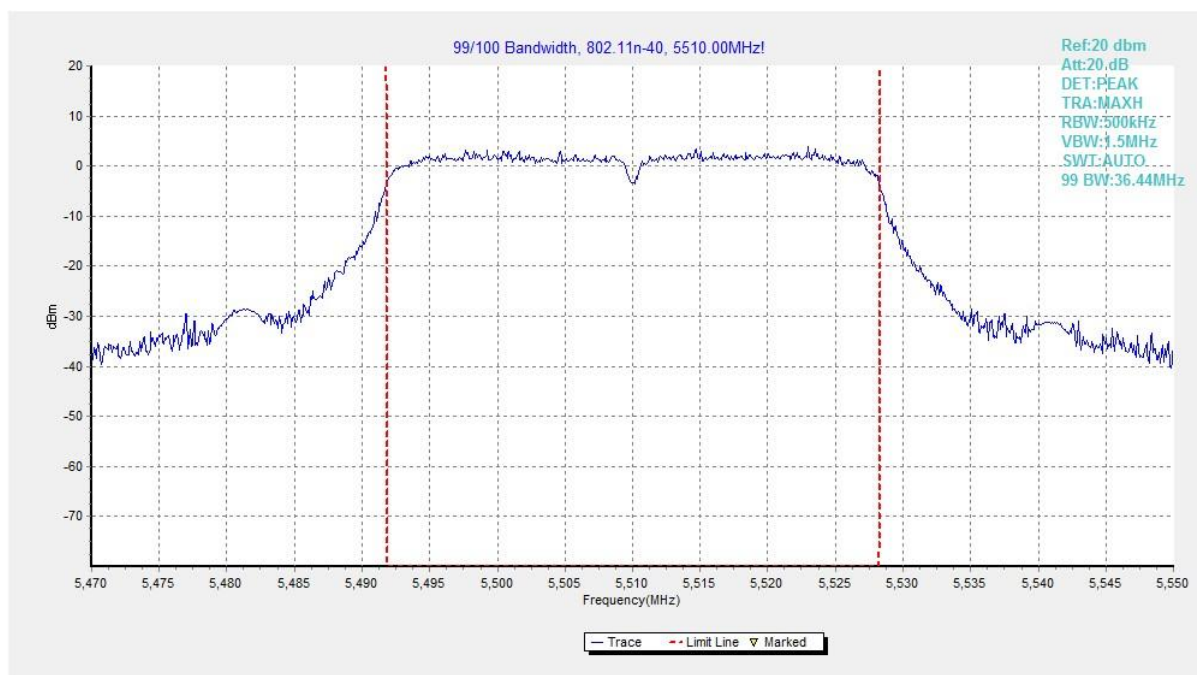
Fig. 35 99% Occupied Bandwidth (802.11n-HT40, 5510MHz)
