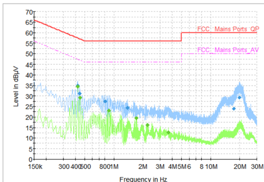
Fig. 75 AC Power line Conducted Emission (Traffic, AE2, 120V)
