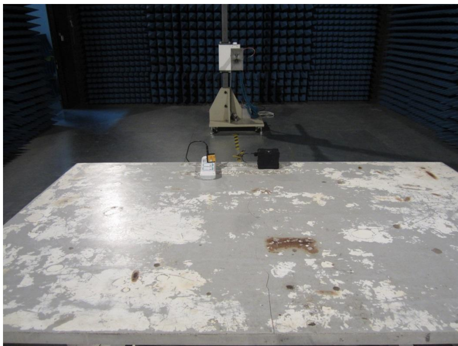
Figure 3 Radiated emission
