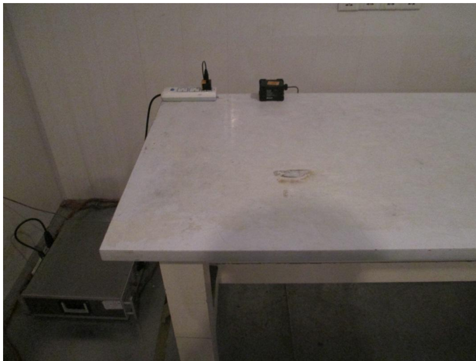
Figure 1 Conducted emission
