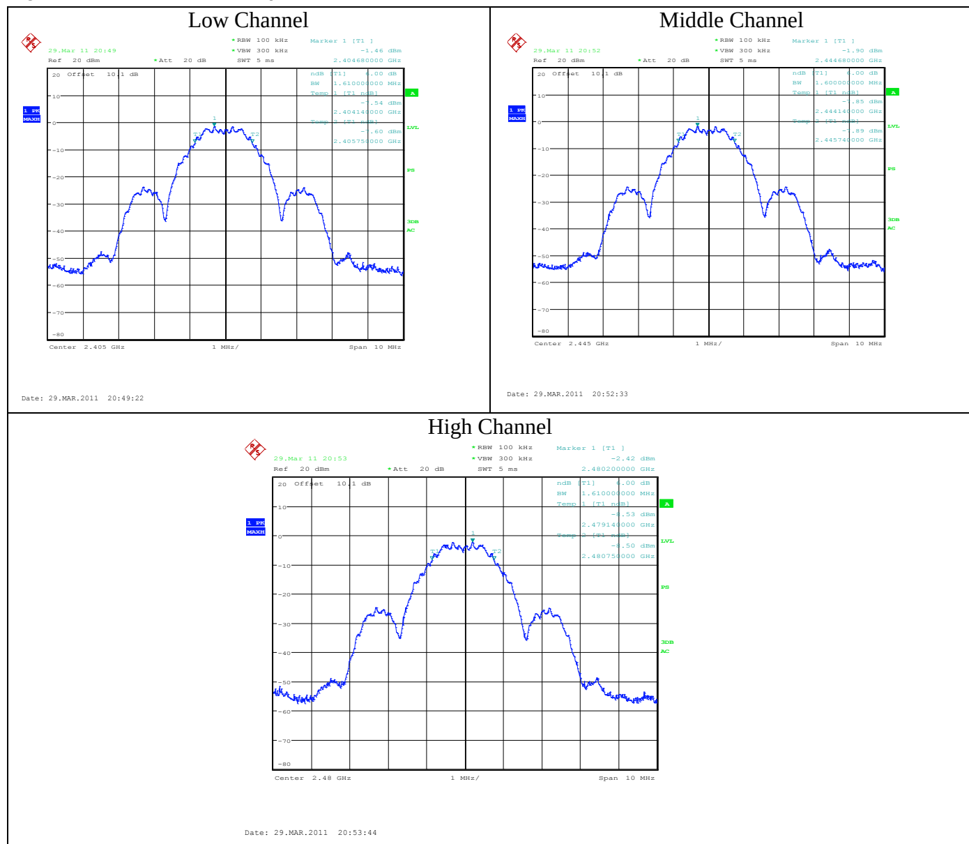
Figure 24 6dB Bandwidth Graphs – Antenna 1
