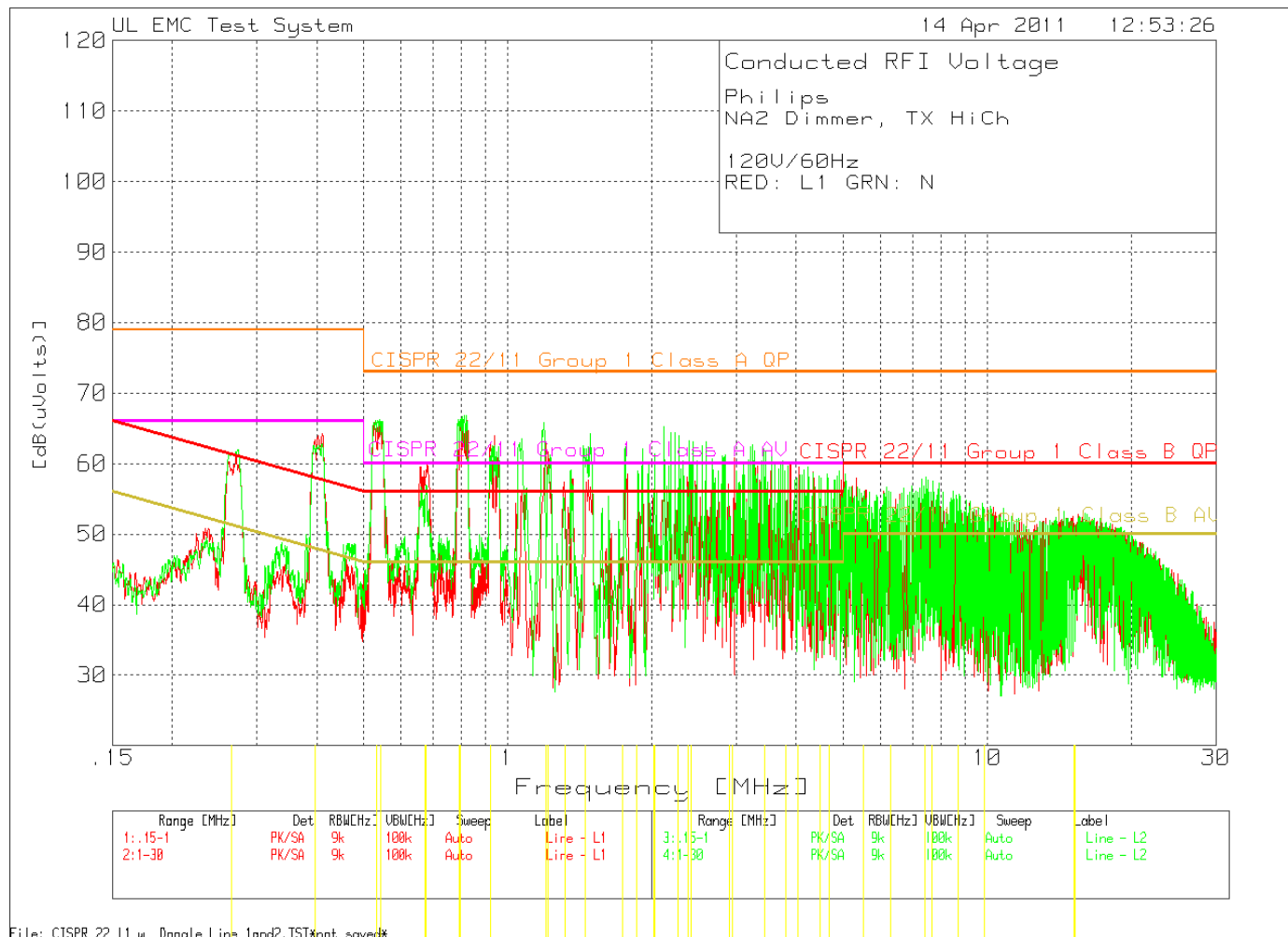
Figure 7 Conducted Emissions Graph – Dimmer – High Channel
