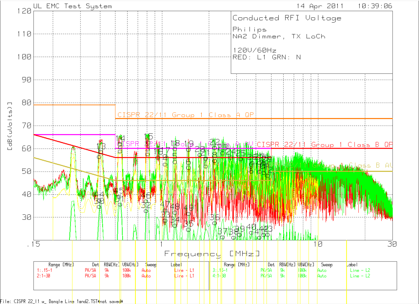
Figure 5 Conducted Emissions Graph – Dimmer – Low Channel
