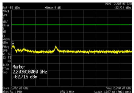
LTE20_16QAM_AWS-4 OBE_2202 to 2290MHz
