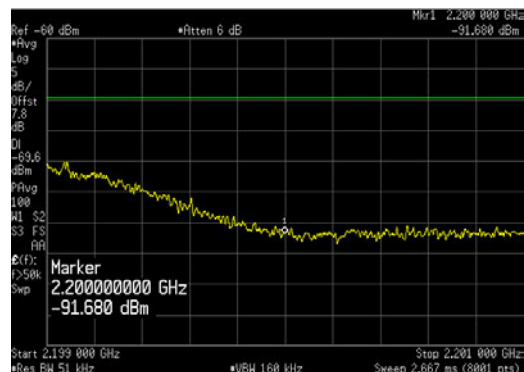
LTE5_QPSK_AWS-4 OBE_2199 to 2201MHz
