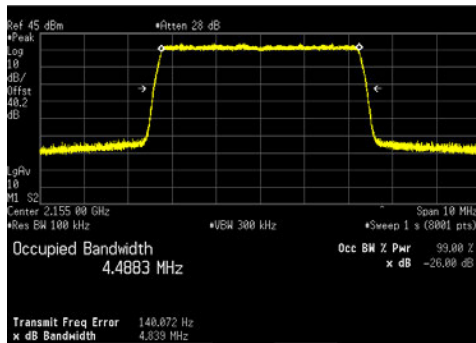
LTE5_QPSK
