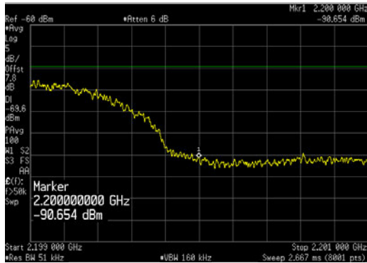
Dual LTE5_QPSK_AWS-4 OBE_2199 to 2201MHz
