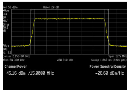
LTE15_Top Channel_Average
