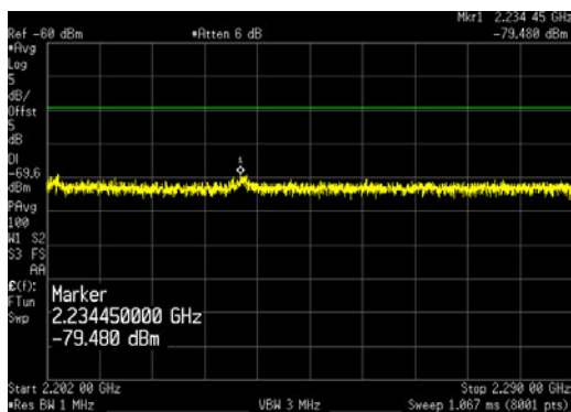
Dual LTE5_QPSK_AWS-4 OBE_2202 to 2290MHz
