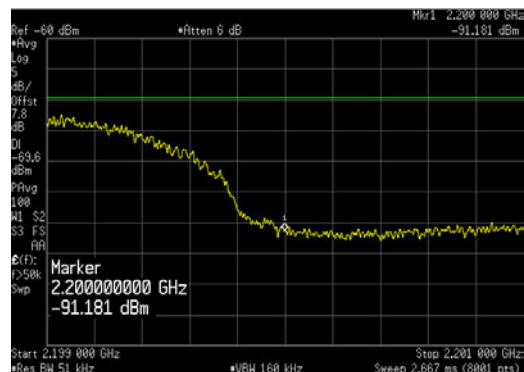
Dual LTE5_64QAM_AWS-4 OBE_2199 to 2201MHz
