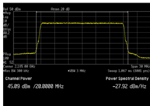
LTE20_Top Channel_Average
