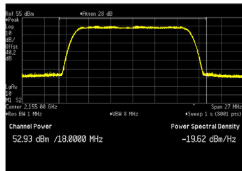
LTE15_Top Channel_Peak
