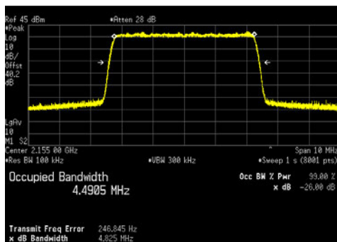
LTE5_64QAM
