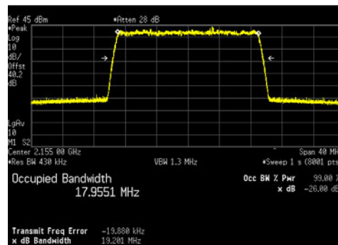
LTE20_16QAM
