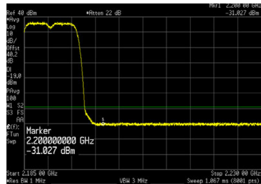
Upper Band Edge_2185 to 2230MHz_256QAM
