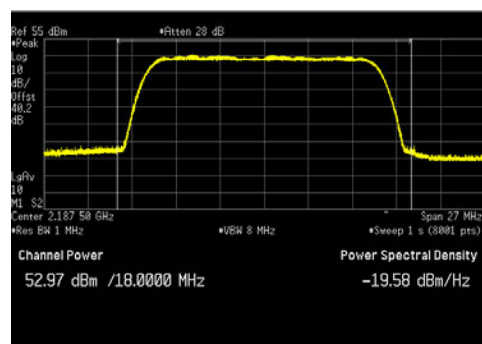
LTE20_Middle Channel_Peak
