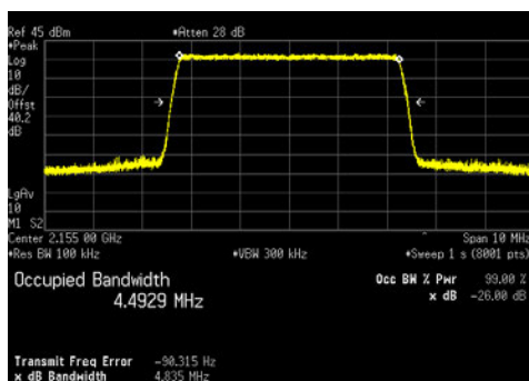
LTE5_256QAM
