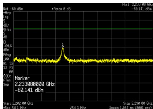
LTE5_64QAM_AWS-4 OBE_2202 to 2290MHz
