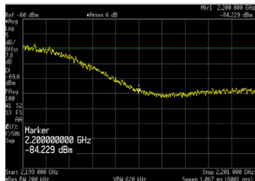
LTE20_64QAM_AWS-4 OBE_2199 to 2201MHz
