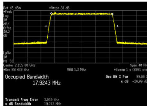
LTE20_QPSK
