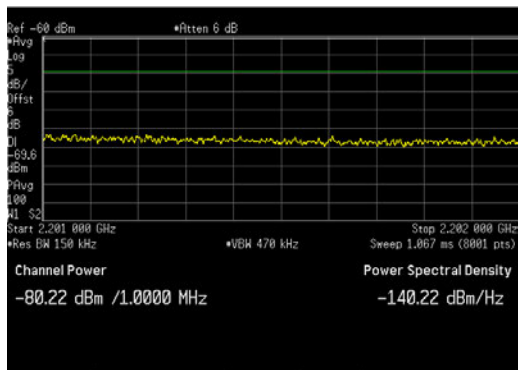
LTE15_64QAM_AWS-4 OBE_2201 to 2202MHz
