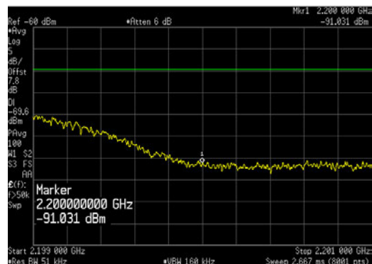
LTE5_64QAM_AWS-4 OBE_2199 to 2201MHz
