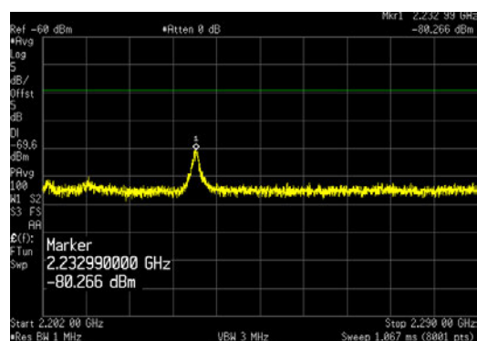
LTE5_16QAM_AWS-4 OBE_2202 to 2290MHz
