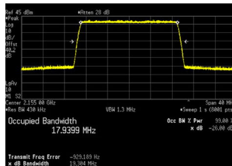
LTE20_64QAM
