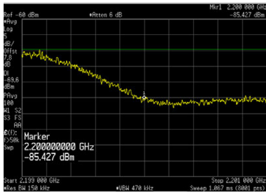
LTE15_64QAM_AWS-4 OBE_2199 to 2201MHz
