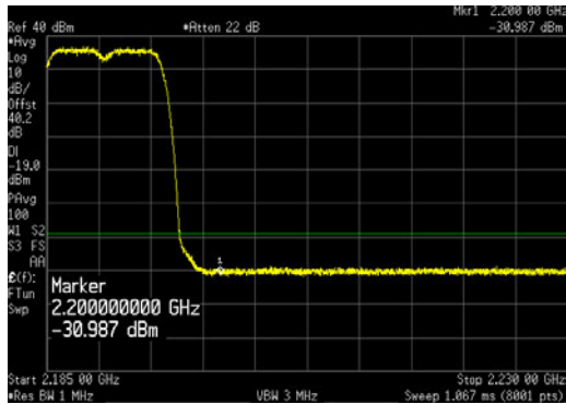
Upper Band Edge_2185 to 2230MHz_QPSK
