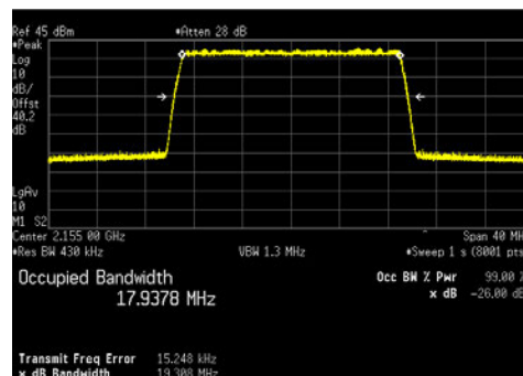
LTE20_256QAM
