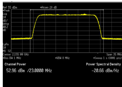
LTE20_Top Channel_Peak
