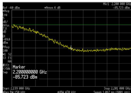
LTE15_QPSK_AWS-4 OBE_2199 to 2201MHz
