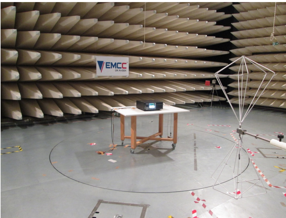
Photo A1-2: Radiated emissions measurement at 3 m distance, 30 MHz – 250 MHz
