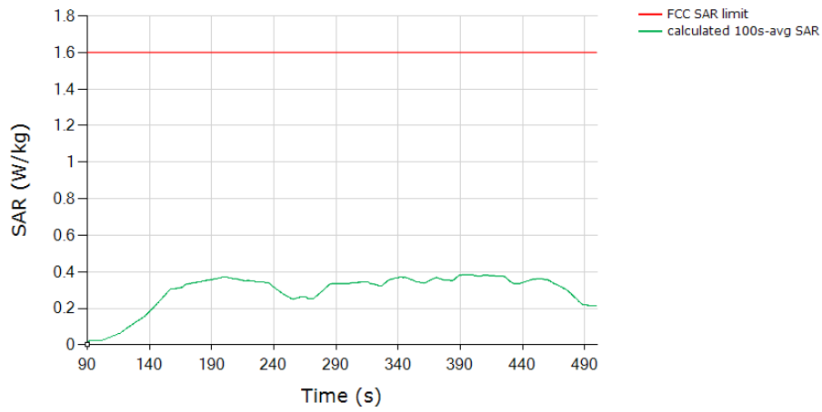
SAR (Test Sequence 2) Tech: NRSUB6SA, Band 41
