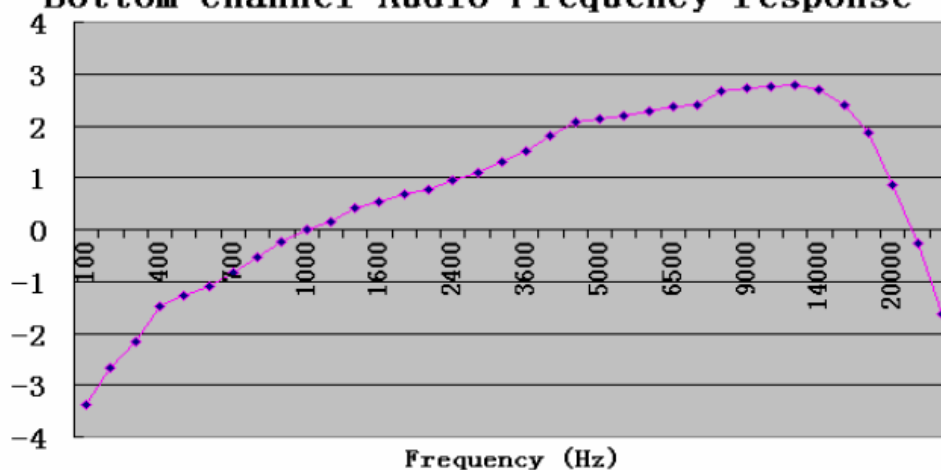
Bottom channel Audio Frequency response
