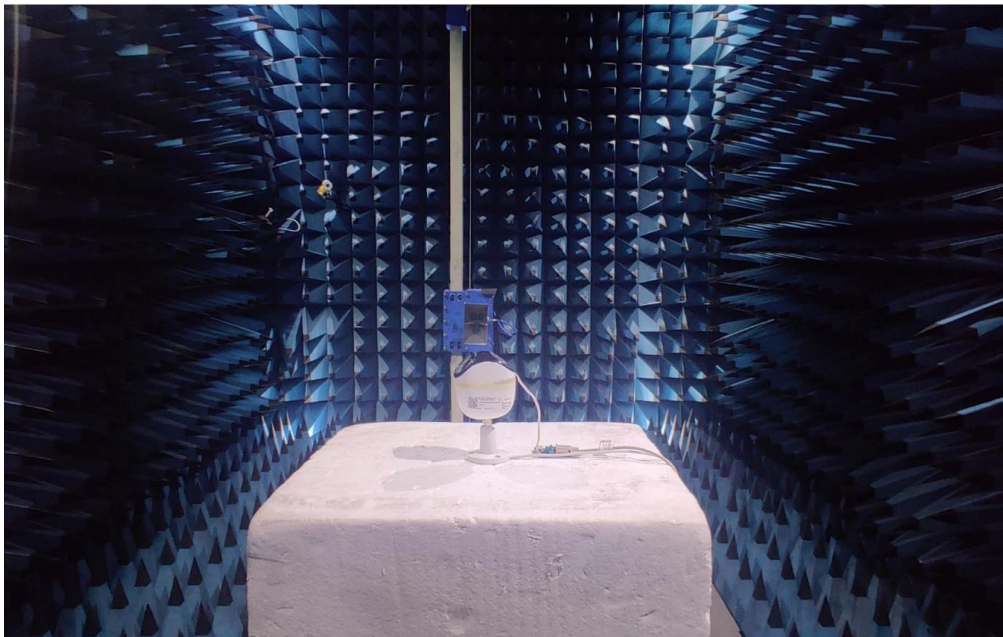
Radiated Emissions Above 1GHz
