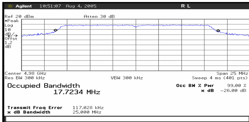
Plot 17. Measured Occupied Bandwidth
