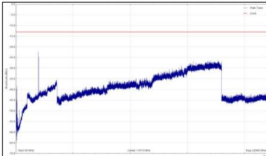
Top - NR&NB-IoT - B25, 1990MHz, 30 MHz to 22 GHz, Vertical (Peak)
