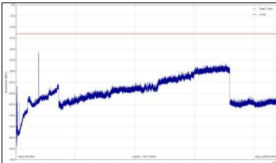
Bot - NR&NB-IoT - B25, 1935MHz, 30 MHz to 22 GHz, Vertical (Peak)
