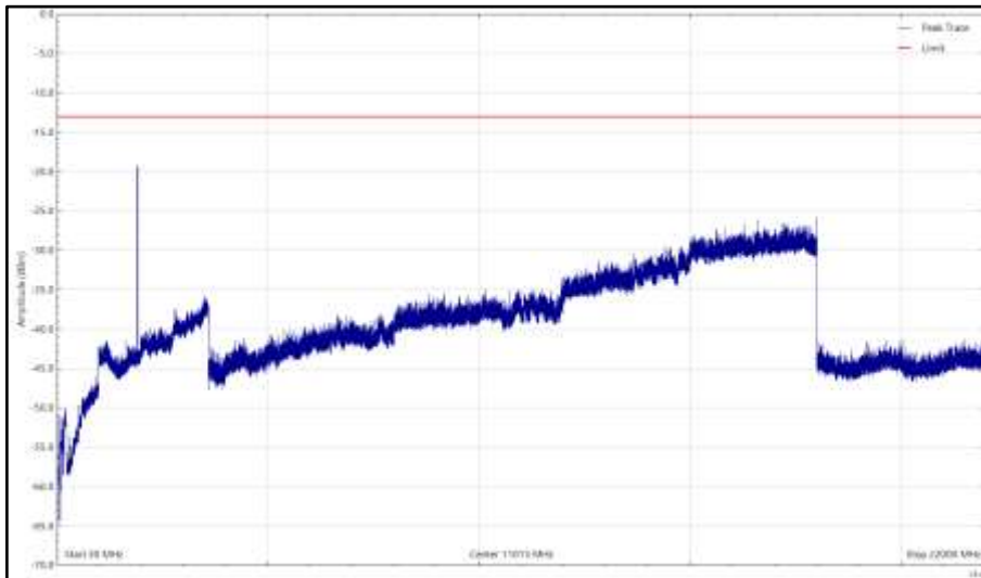
Bot - NR&NB-IoT - B25, 1935MHz, 30 MHz to 22 GHz, Horizontal (Peak)
