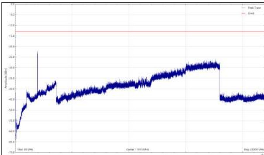
Mid - NR&NB-IoT - B25, 1962.5MHz, 30 MHz to 22 GHz, Vertical (Peak)
