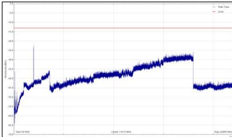
Top - NR&NB-IoT - B25, 1990MHz, 30 MHz to 22 GHz, Horizontal (Peak)
