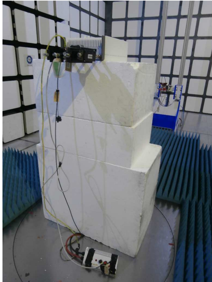
Radiated Emissions 1 GHz to 12 GHz
