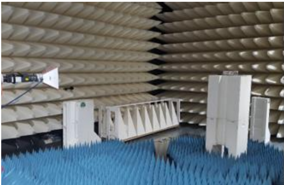
Figure B4. Radiated Emission High Range 1-18GHz test setup
