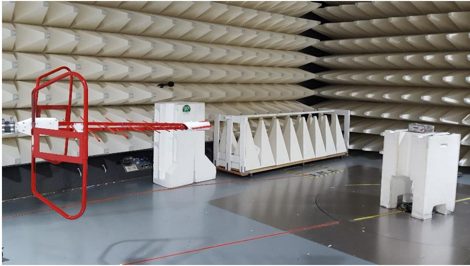
Figure B3. Radiated Emission Low Range test setup
