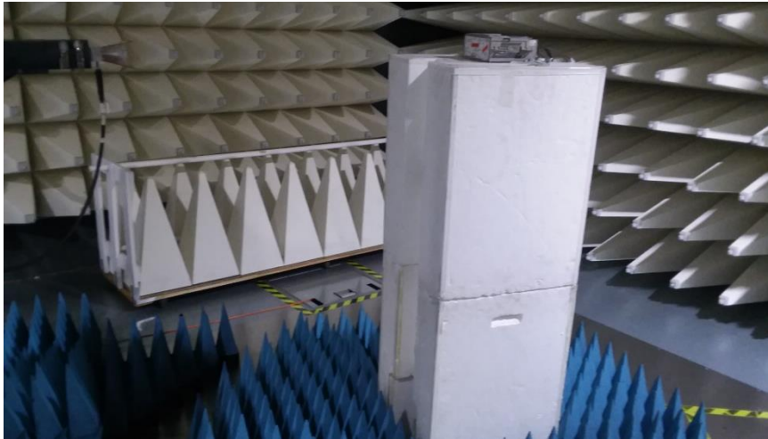
Figure B5. Radiated Emission High Range 18-40GHz test setup
