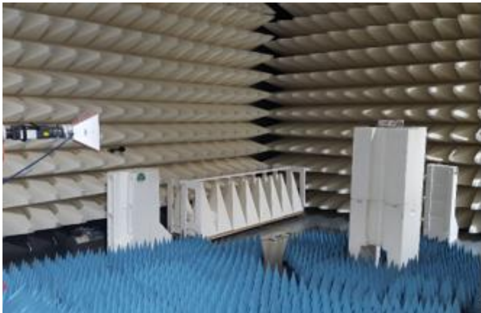
Figure C4. Radiated Emission High Range 1-18GHz test setup
