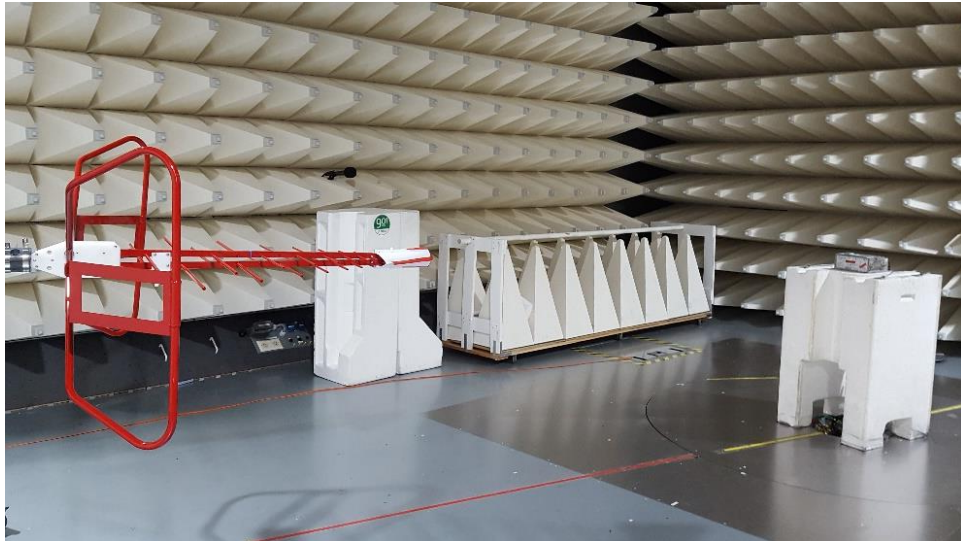
Figure C3. Radiated Emission Low Range test setup
