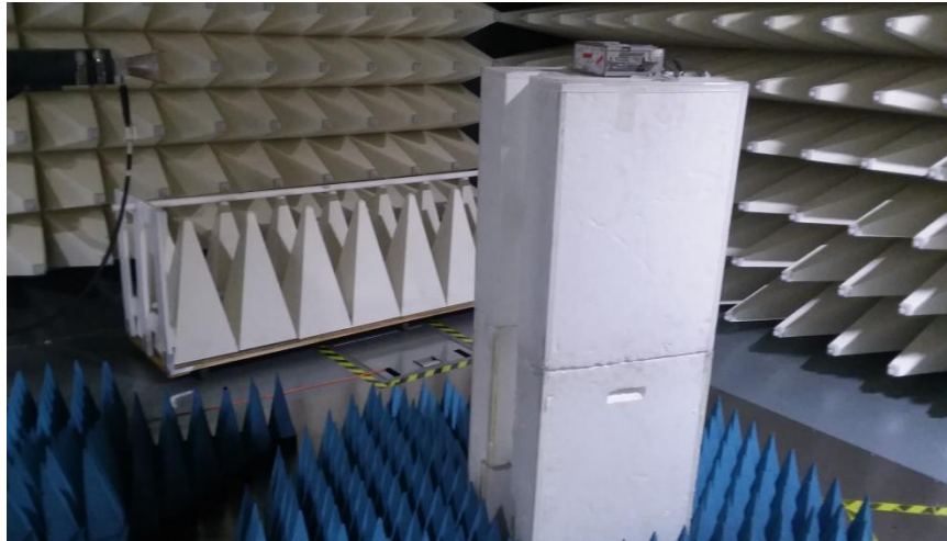
Figure C5. Radiated Emission High Range 18-40GHz test setup
