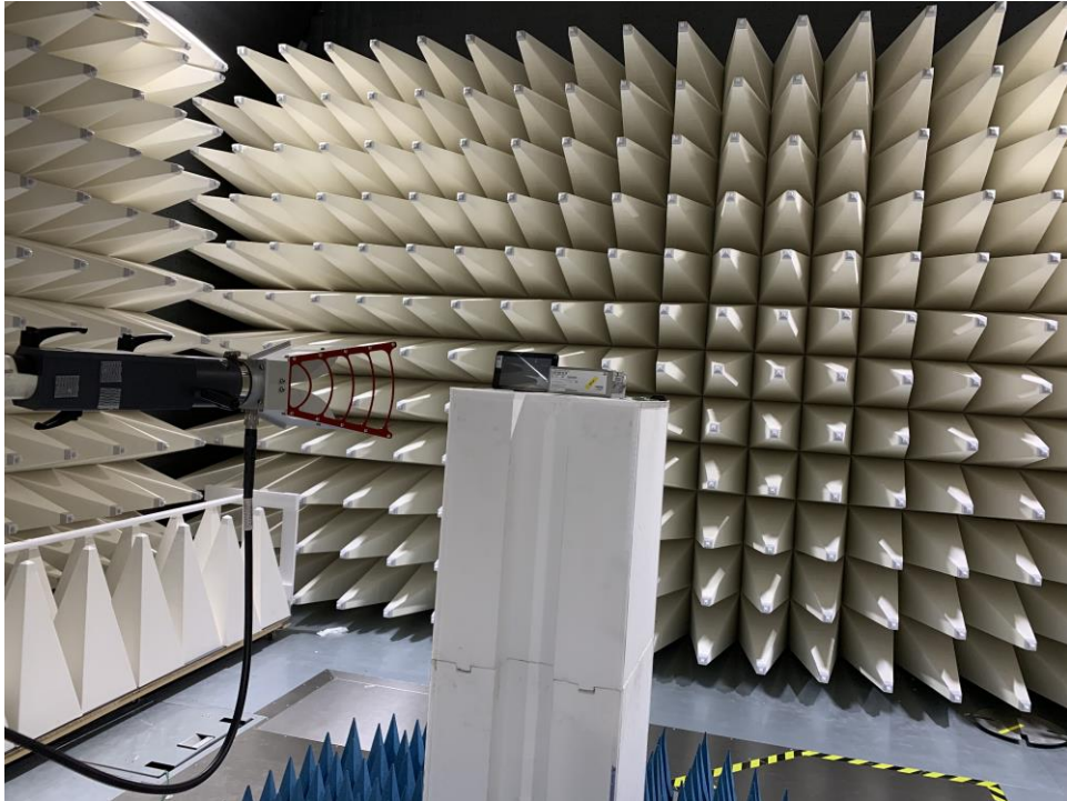
Figure C3. Radiated Setup – High Range
