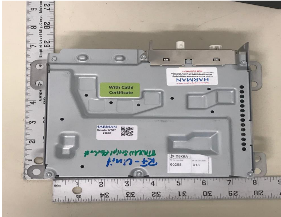
Figure C1: Head Unit
