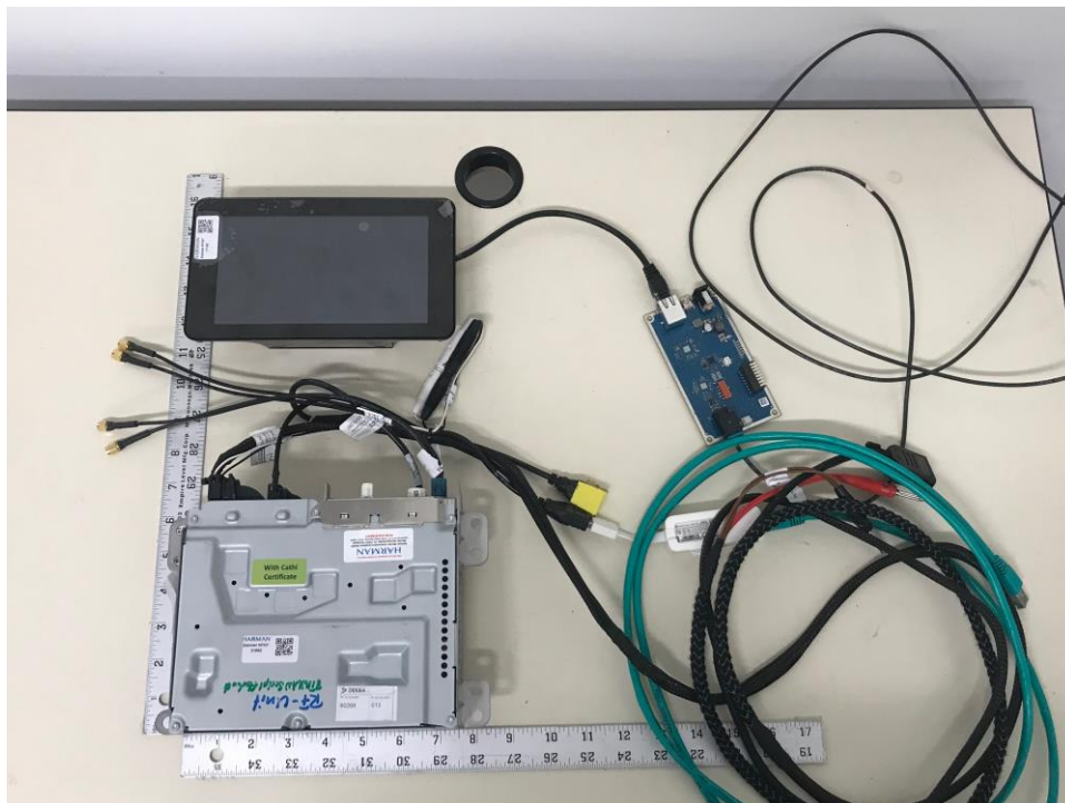
Figure C2: Conducted DUT Set up
