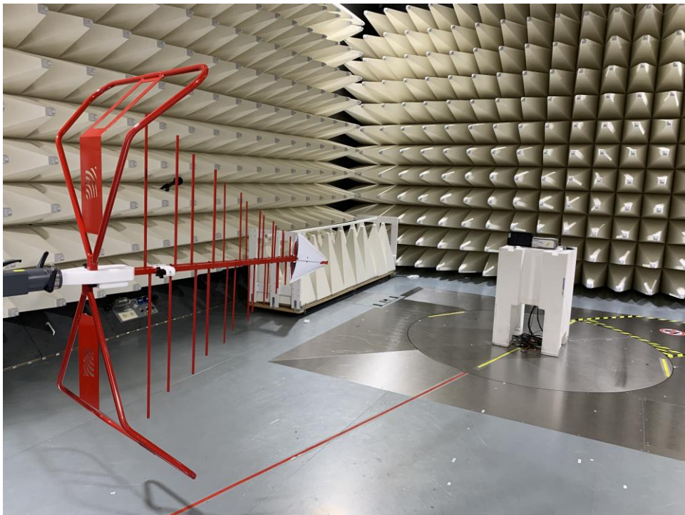
Figure C4. Radiated Setup – Low Range
