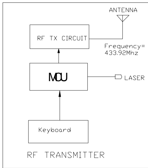
Transmitter Block Diagram
