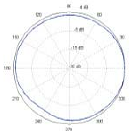
Azimuth
