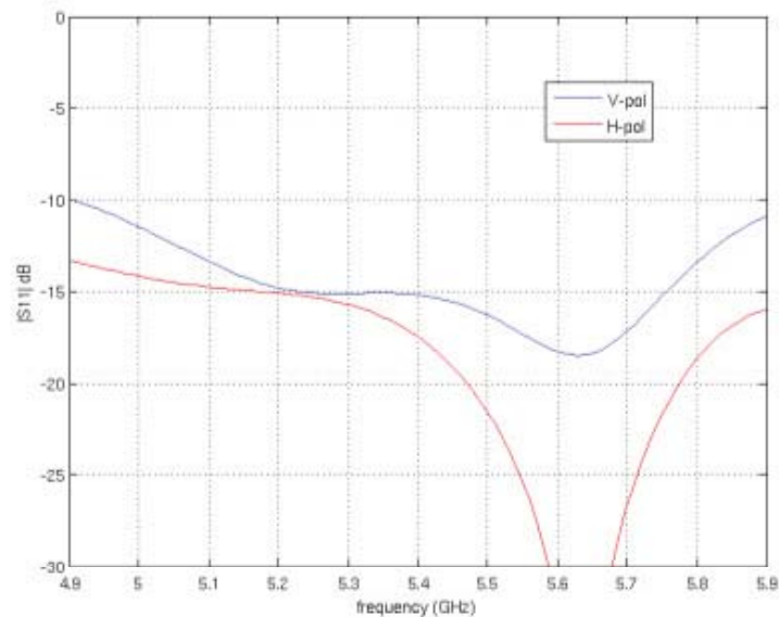
Return Loss
