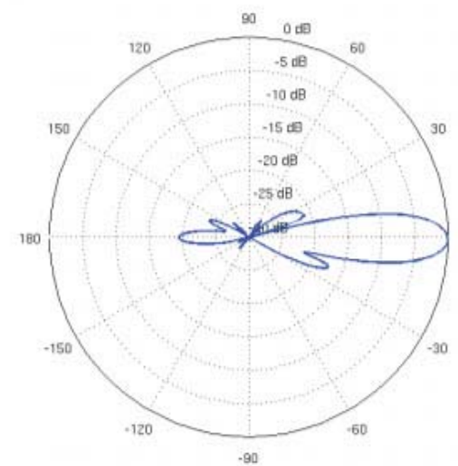
Vertical Elevation
