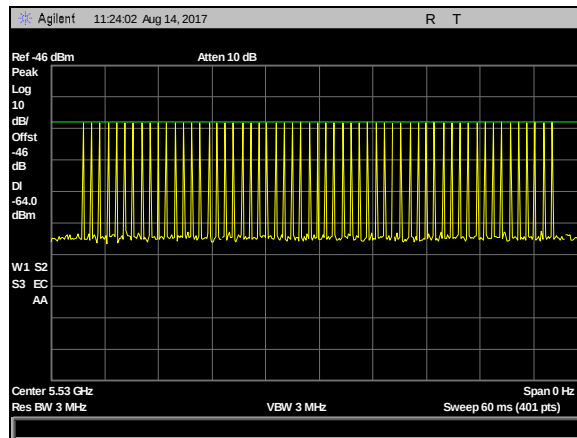
Plot 47. DFS Calibration Plots, Type 1 Calibration 5530 MHz, Sig Gen Level -23 dBm
