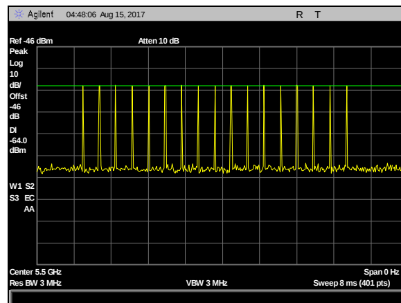
Plot 32. DFS Calibration Plots, Type 3 Calibration 5500 MHz, Sig Gen Level -23 dBm
