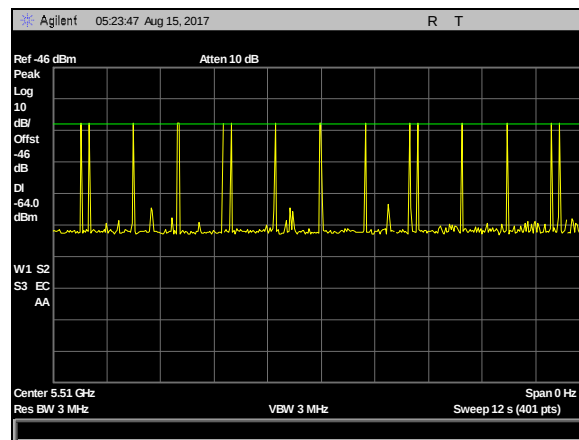
Plot 14. DFS Calibration Plots, Type 5 Calibration 5510 MHz, Sig Gen Level -23 dBm
