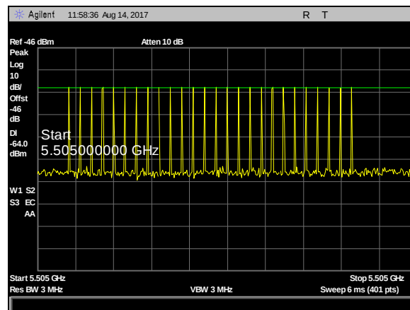
Plot 41. DFS Calibration Plots, Type 2 Calibration 5505 MHz, Sig Gen Level -23 dBm
