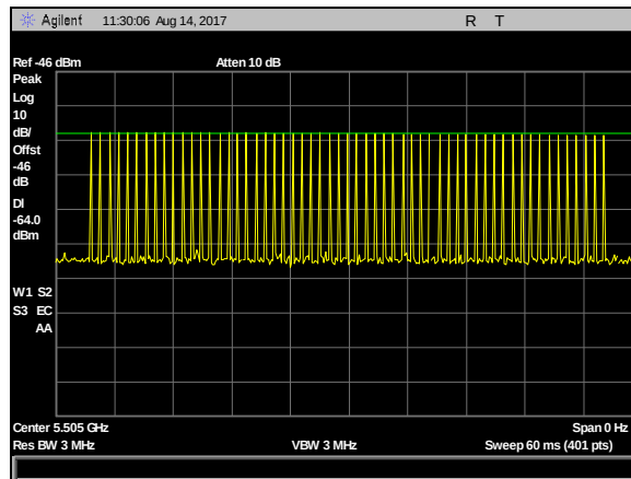
Plot 44. DFS Calibration Plots, Type 1 Calibration 5505 MHz, Sig Gen Level -23 dBm
