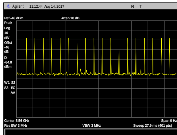
Plot 50. DFS Calibration Plots, Type 0 Calibration 5560 MHz, Sig Gen Level -23 dBm
