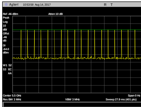
Plot 56. DFS Calibration Plots, Type 0 Calibration 5500 MHz, Sig Gen Level -23 dBm
