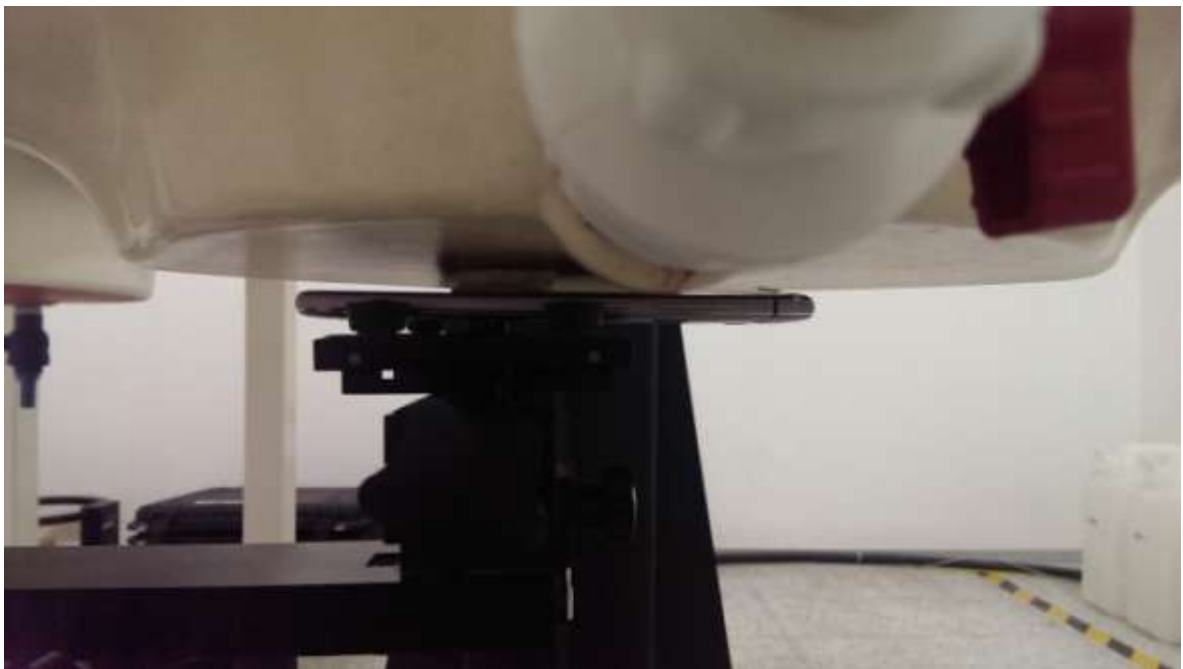
POSITION OF BODY TOWARDS PHANTOM WITH 10mm DISTANCE
