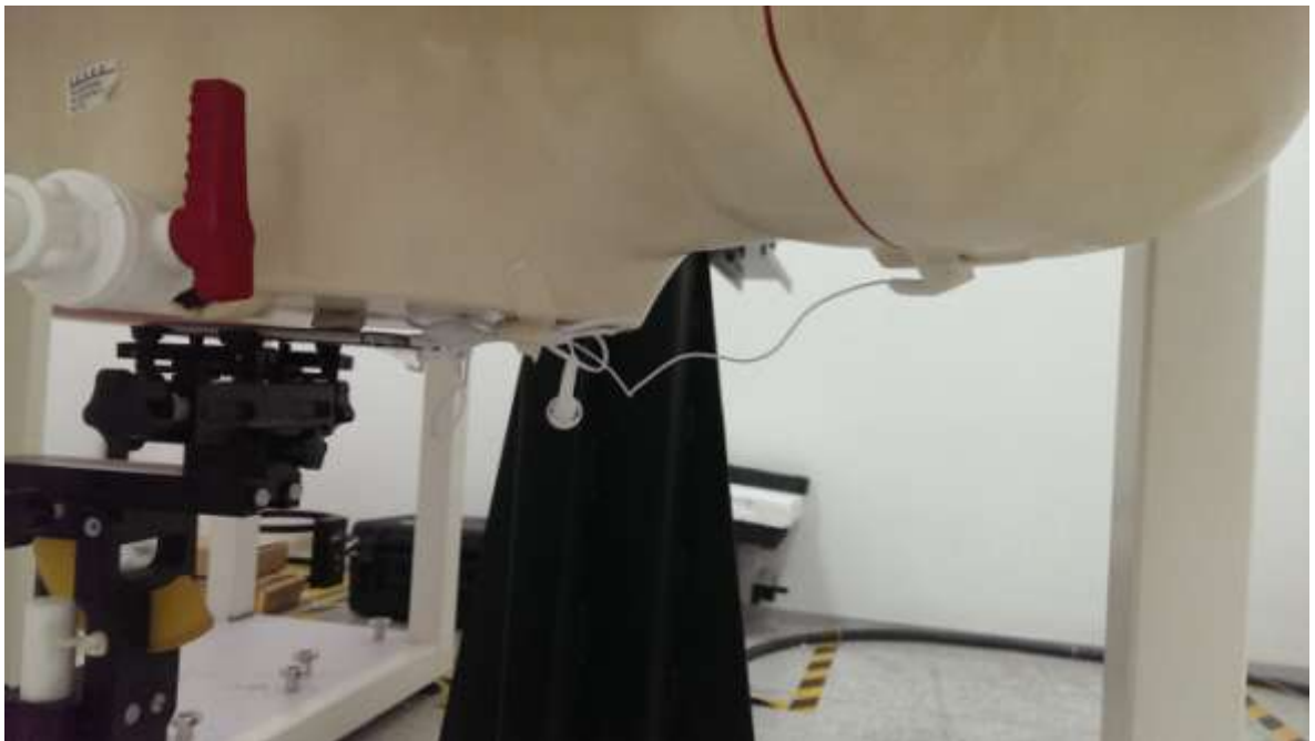
POSITION OF BODY TOWARDS GROUND WITH 10mm DISTANCE (WITH EARPHONE)
