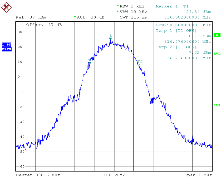
(Plot C4: EDGE 850MHz Channel = 190 99% Occupied Bandwidth)
