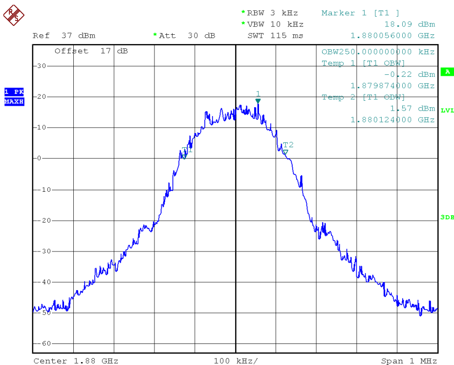
(Plot D4: EDGE 1900MHz Channel = 661 99% Occupied Bandwidth)
