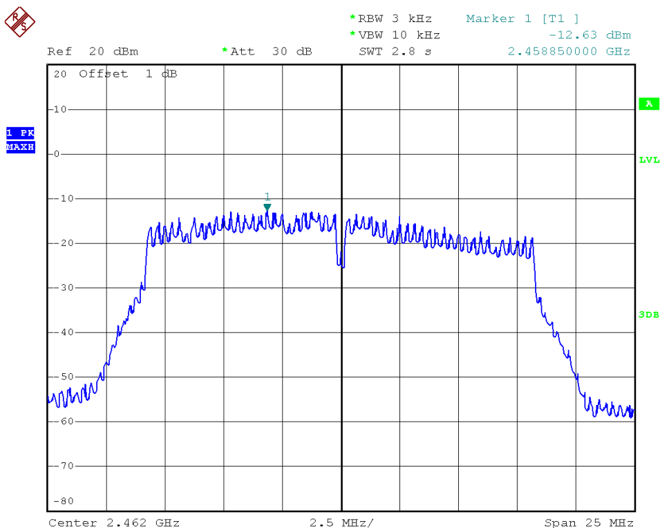
802.11g - Channel 11
