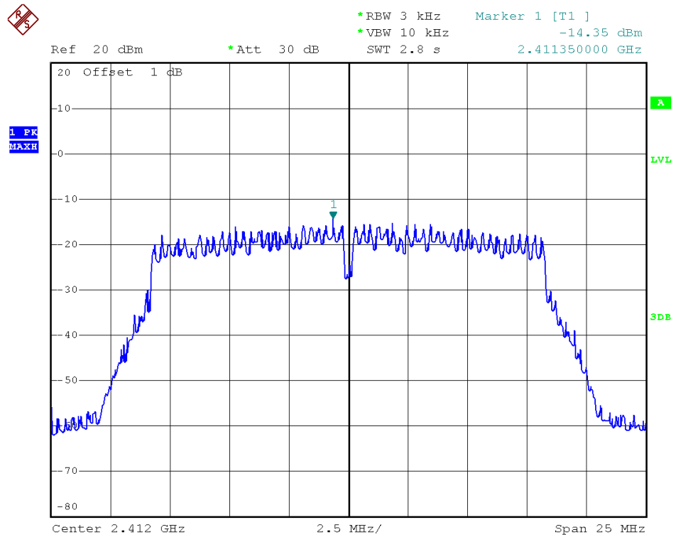
802.11g - Channel 1
