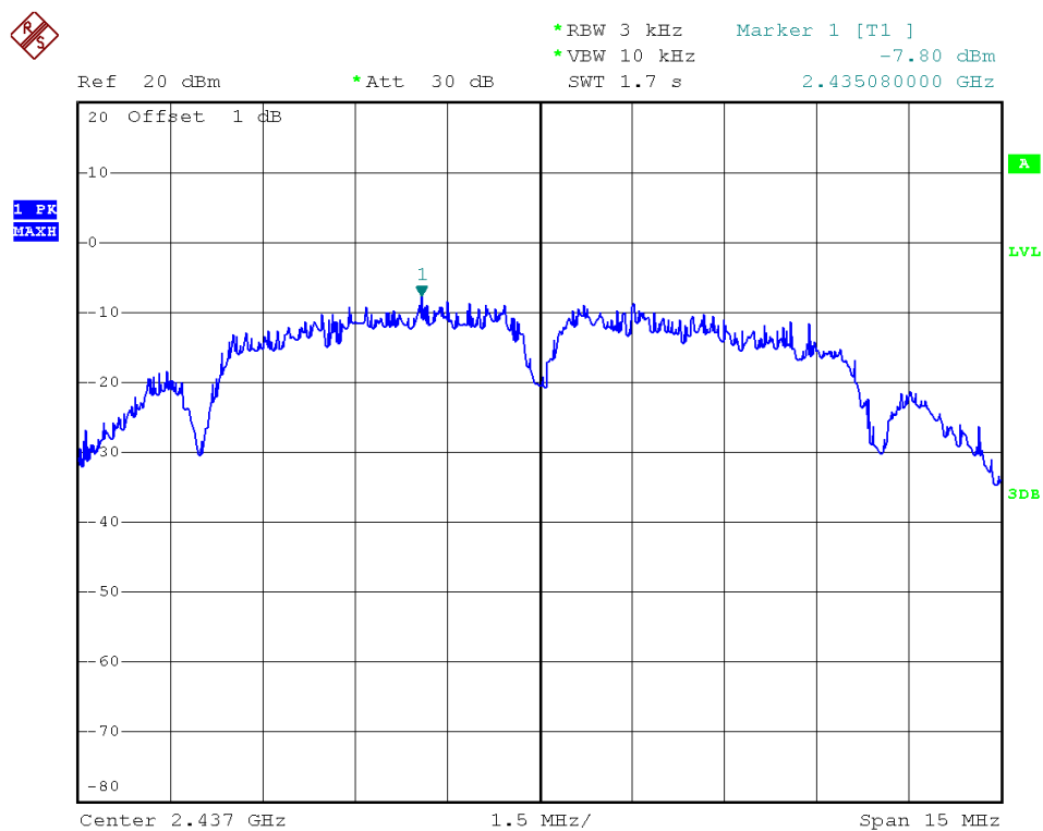
802.11b - Channel 6
