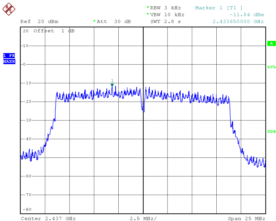
802.11n20 - Channel 6
