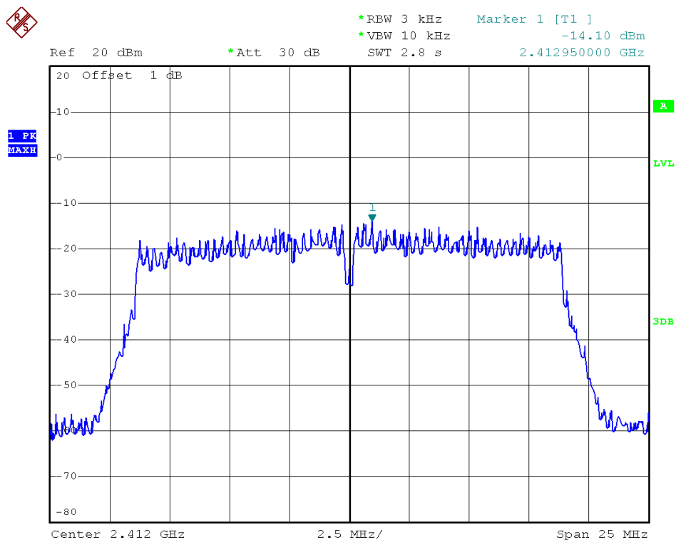
802.11n20 - Channel 1
