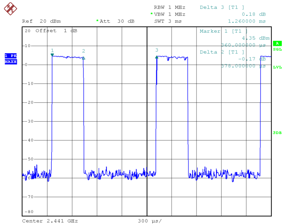
39 Channel @ 2DH1
