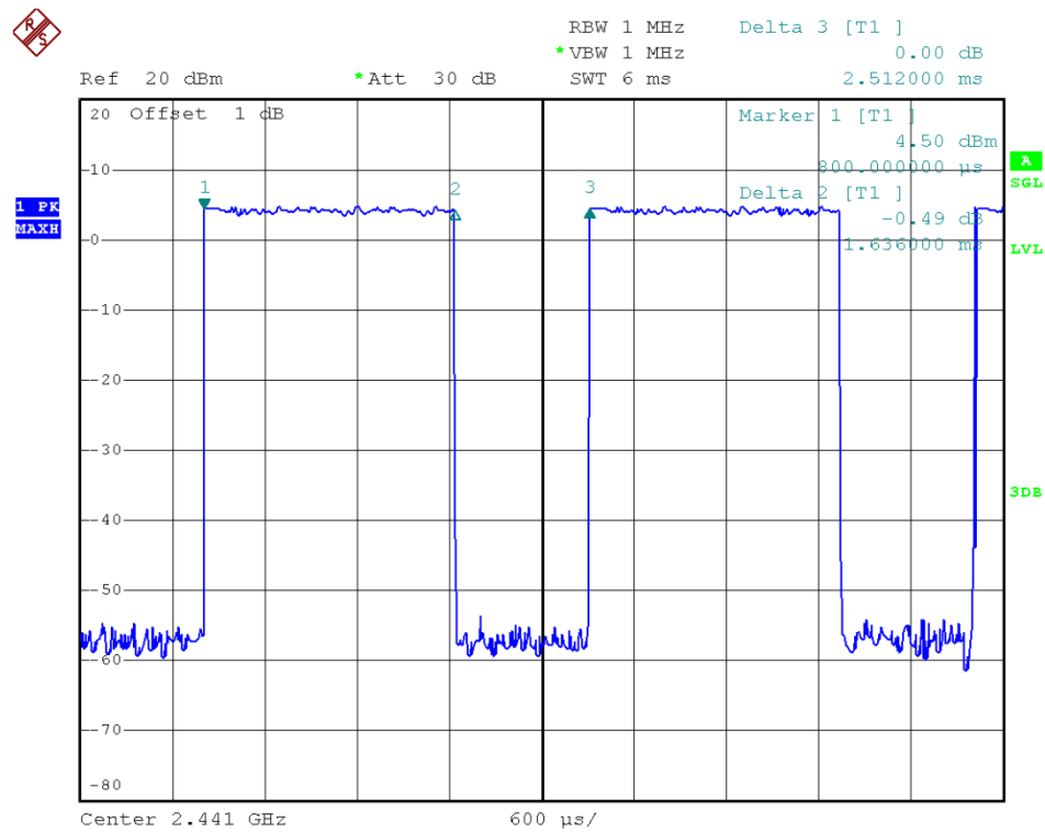
39 Channel @ 3DH3
