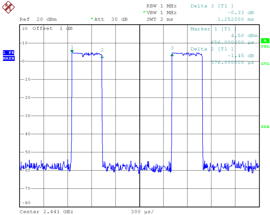
39 Channel @ 3DH1
