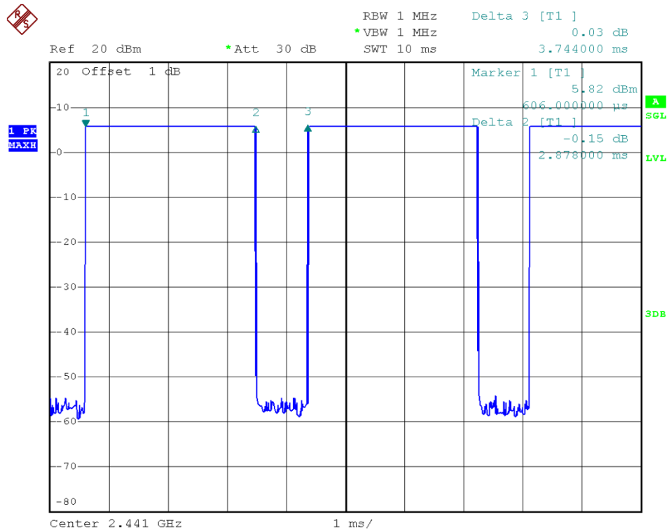
39 Channel @ DH5
