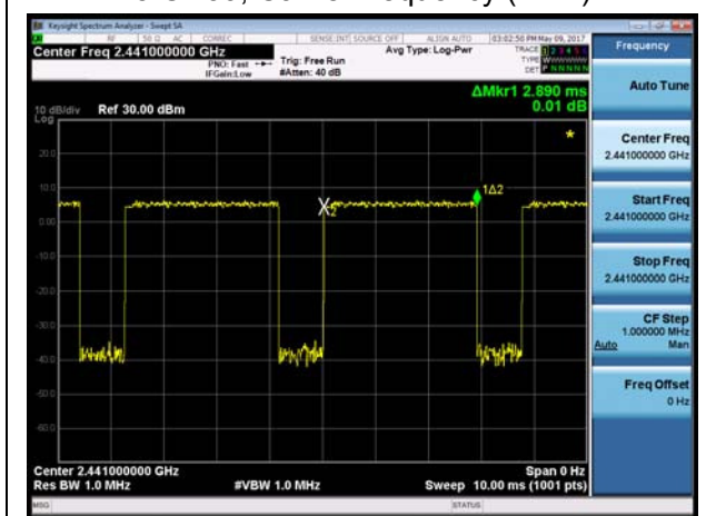
BT DH5 CH39, Carrier frequency (MHz): 2441
