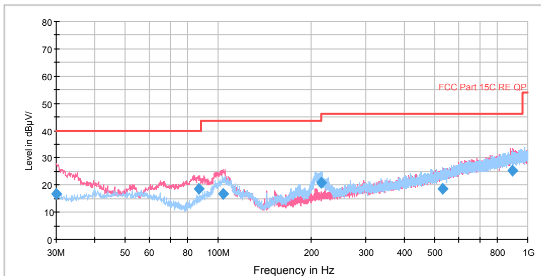
FCC RE 0.03-1GHz QP Class B
