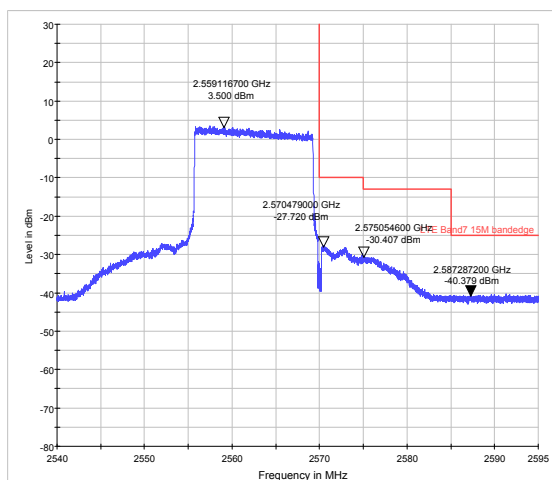
LTE Band 7 QPSK 15MHz CH-High, RB 75
