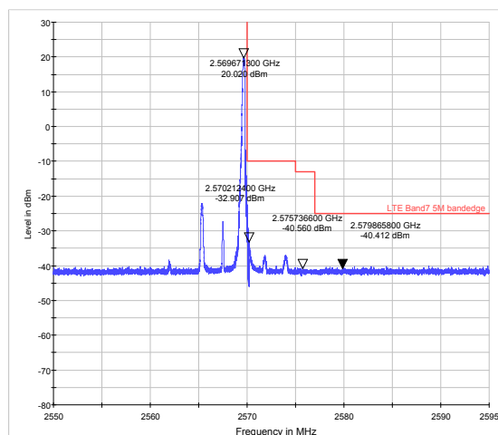
LTE Band 7 QPSK 5MHz CH-High, RB 25
