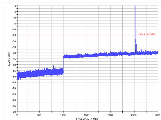
LTE Band 7 5MHz CH-Middle 30MHz~3GHz
