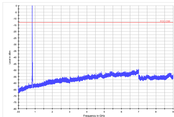
WCDMA Band V CH-Low 30MHz~9GHz
