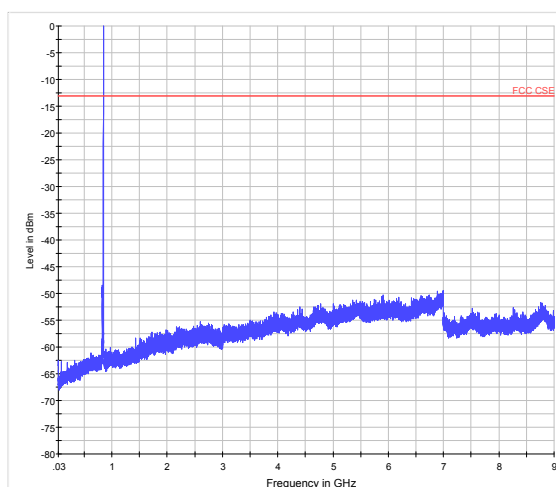
WCDMA Band V CH-High 30MHz~9GHz
