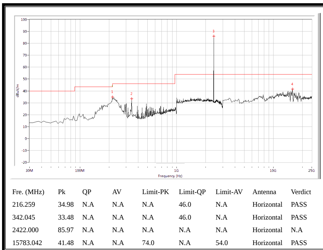
(Plot A.2: Antenna Horizontal, 30MHz to 25GHz)
