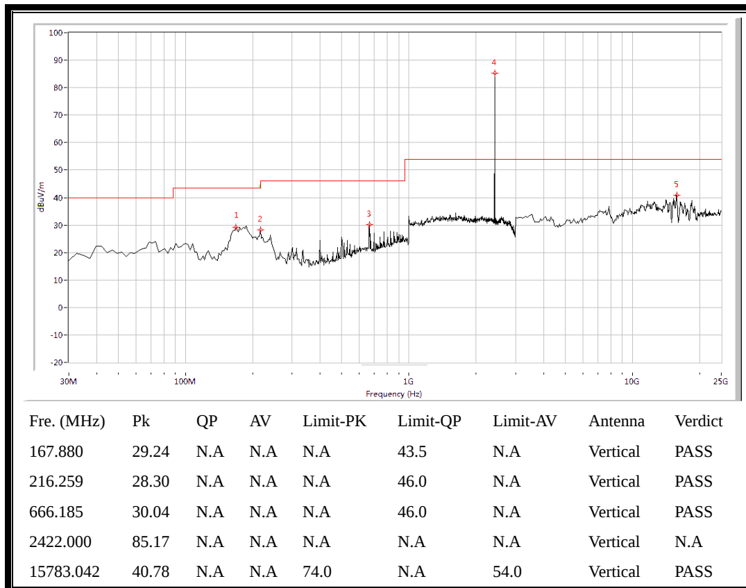
(Plot A.3: Antenna Vertical, 30MHz to 25GHz)
