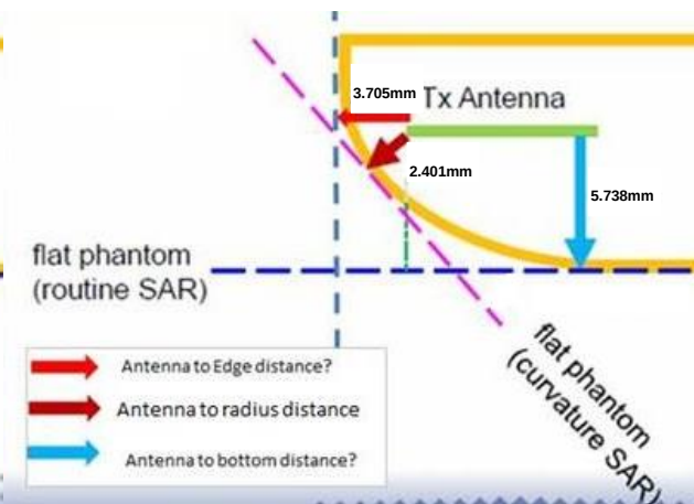
X=3.705mm, Y=5.738mm, Z=2.401mm Exterior Radius Dimension for WLAN
