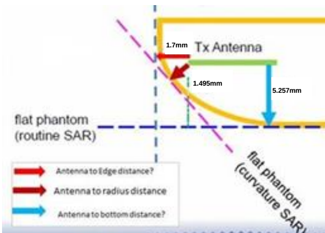
X=1.7mm, Y=5.257mm, Z=1.495mm Exterior Radius Dimension for WWAN
