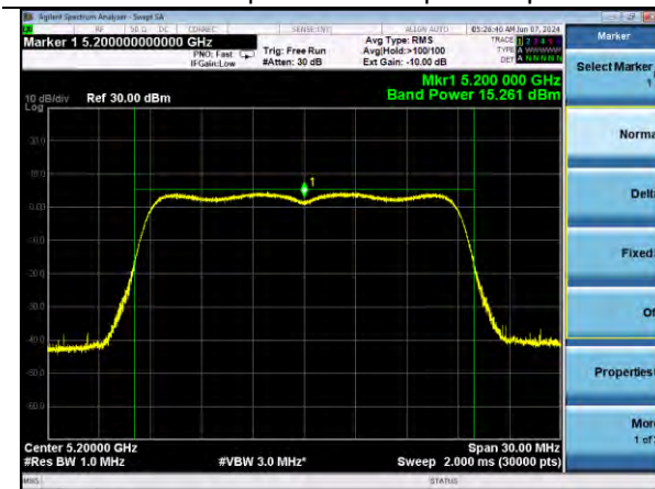
802.11ac20 | Channel 40 | MCS0
