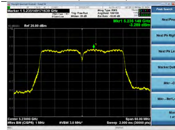
802.11n40 | Channel 46 | MCS7
