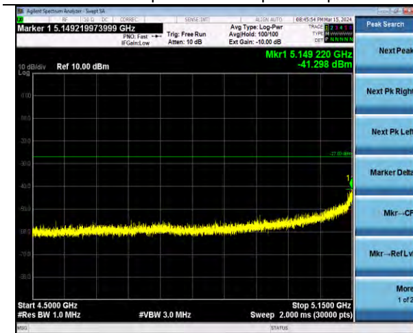
802.11ac40 | Channel 38 | MCS0 | Peak
