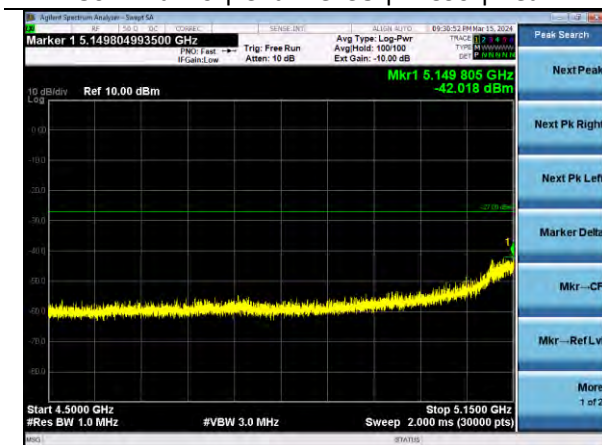
802.11ac80 | Channel 58 | MCS0 | Peak
