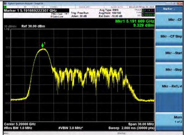
802.11ac20 | Channel 40 | MCS0 | RU26
