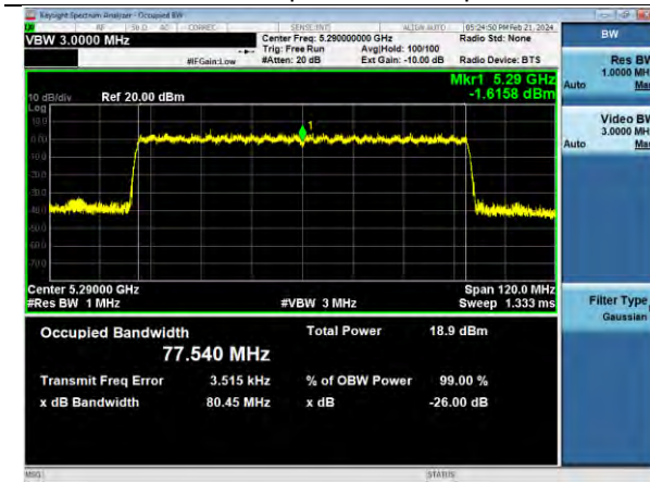
802.11ax80 | Channel 58 | MCS0
