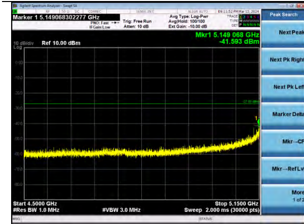
802.11ax40 | Channel 38 | MCS0 | Peak
