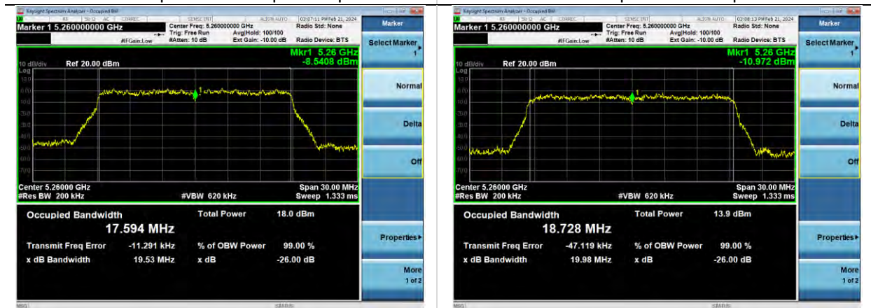
802.11ac20 | Channel 52 | MCS8
