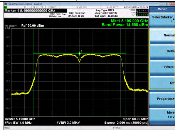
802.11ac40 | Channel 38 | MCS7
