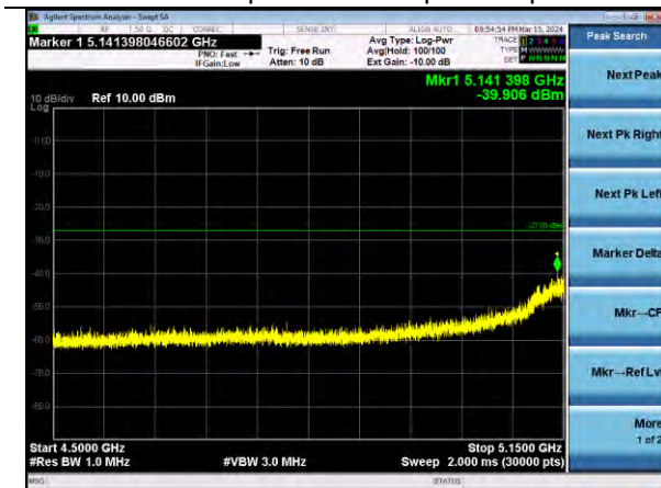
802.11ax80 | Channel 42 | MCS7 | Peak
