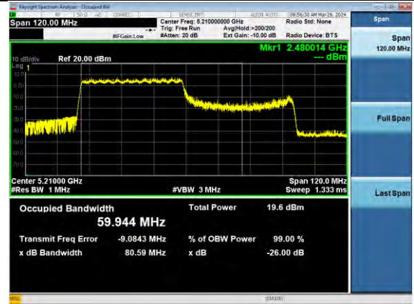
802.11ax80 | Channel 42 | MCS0 | RU Tone 484 Index 65
