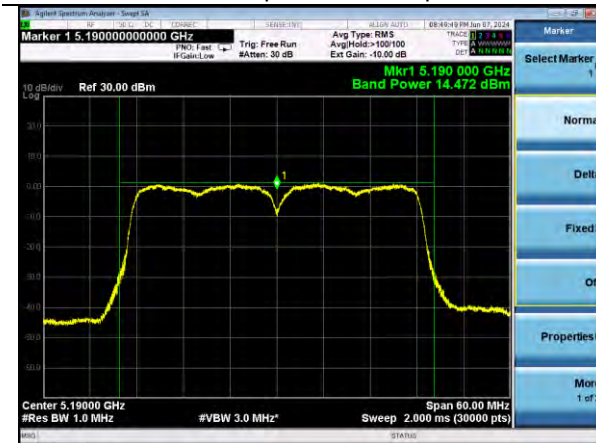
802.11n40 | Channel 38 | MCS7
