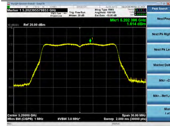
802.11a | Channel 40 | 6 Mbps
