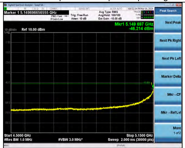
802.11ax20 | Channel 38 | MCS0 | Average
