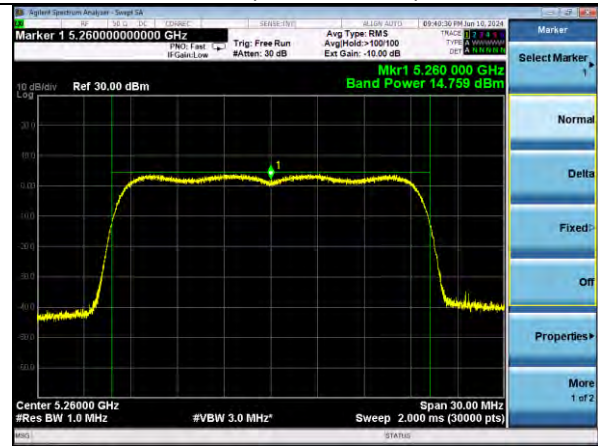
802.11ax20 | Channel 52 | MCS0
