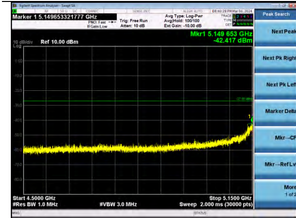
802.11ax20 | Channel 36 | MCS0 | Peak
