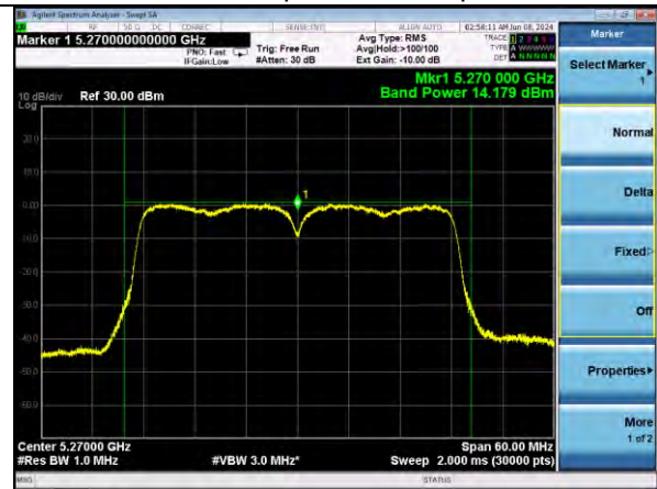
802.11ac40 | Channel 54 | MCS7
