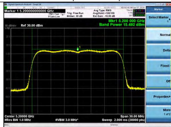
802.11ax20 | Channel 40 | MCS0
