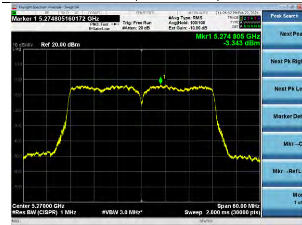
802.11n40 | Channel 54 | MCS7
