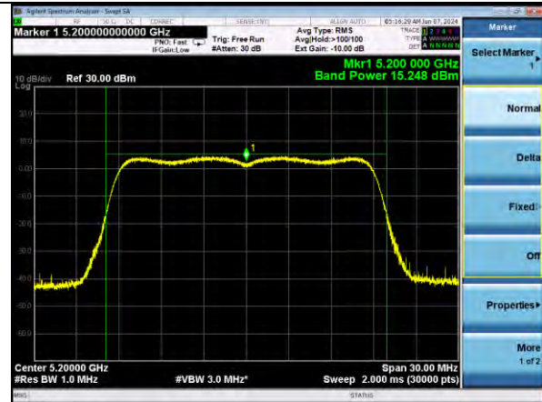
802.11n20 | Channel 40 | MCS0
