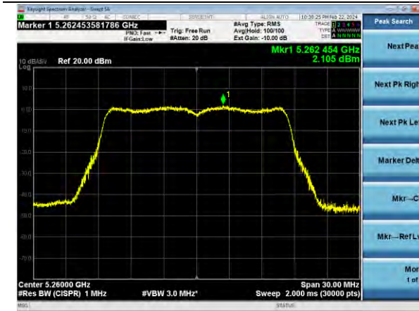
802.11a | Channel 52 | 54 Mbps
