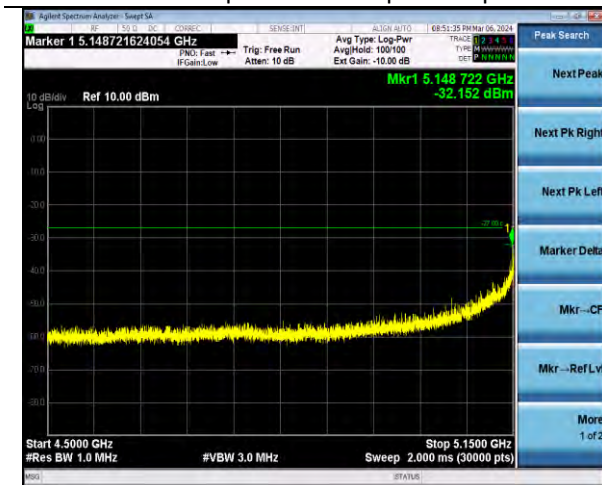
802.11n40 | Channel 38 | MCS0 | Peak
