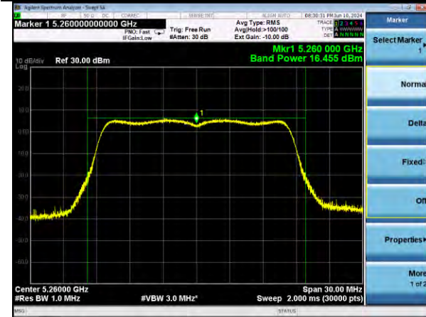
802.11a | Channel 52 | 6 Mbps
