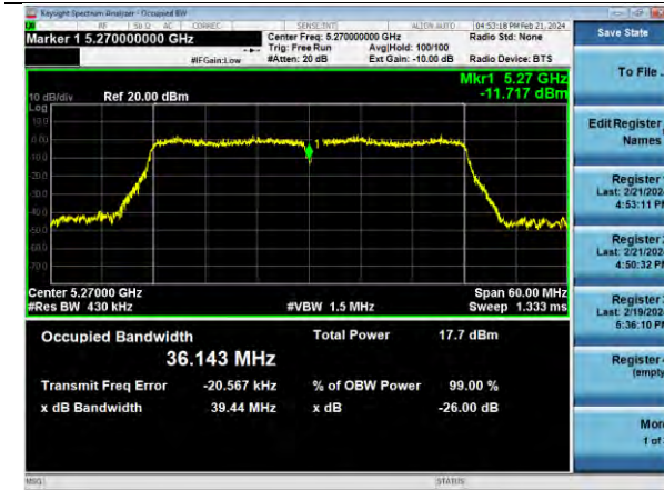
802.11n40 | Channel 54 | MCS7
