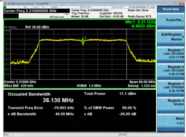
802.11ac40 | Channel 62 | MCS0
