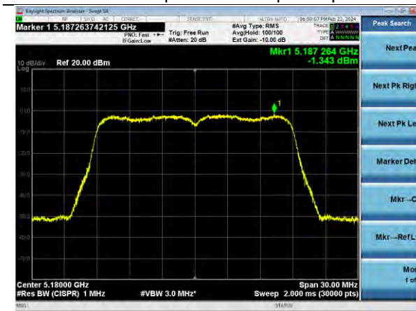
802.11ac20 | Channel 36 | MCS8
