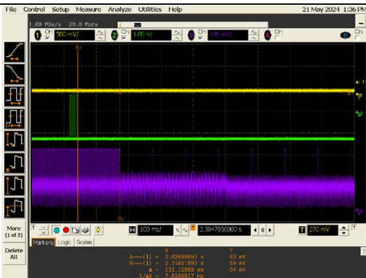
10 beacons after transmissions end at 131ms 467\mu\text{sec} * 10 = 4.67\text{ms} (Require
