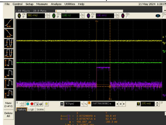
Individual Beacon 467μsec
