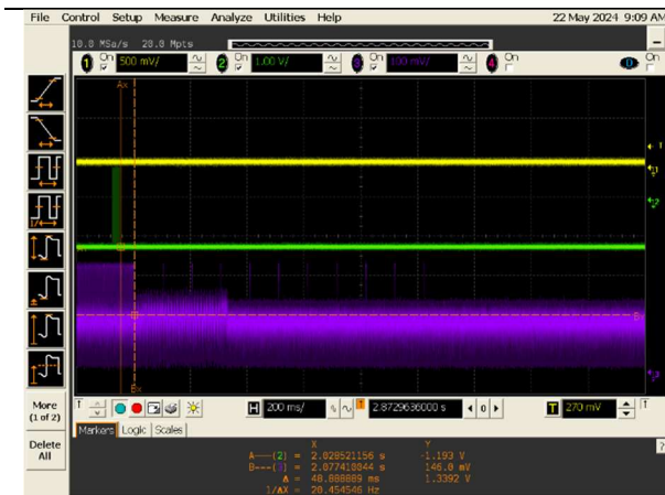
10 beacons after transmissions end at 131ms 467\mu\text{sec} * 10 = 4.7\text{ms} (Require
