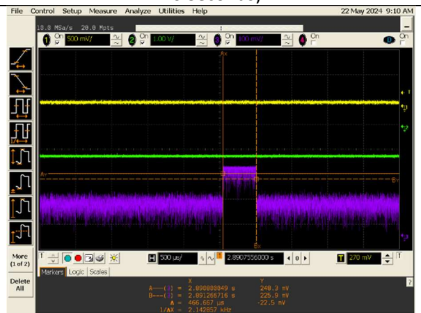
Individual Beacon 467μsec
