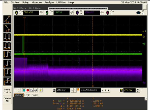
Channel Move Time: 1.1 Seconds (Required Max 10 Seconds)
