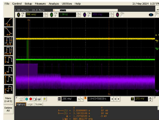
Channel Move Time: 1.2 Seconds (Required Max 10 Seconds)
