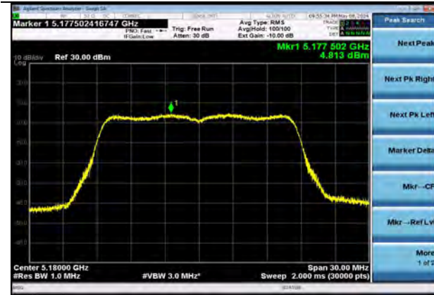
802.11a | Channel 36 | 54 Mbps
