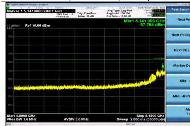
802.11ax80 | Channel 42 | MCS7 | Peak
