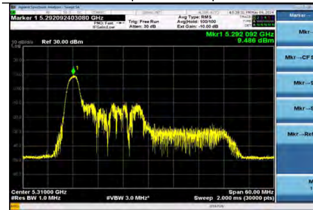
802.11ax40 | Channel 62 | MCS0 | RU26
