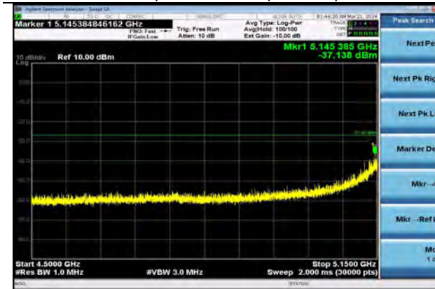
802.11ac40 | Channel 38 | MCS0 | Peak
