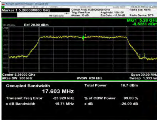
802.11ac20 | Channel 52 | MCS0
