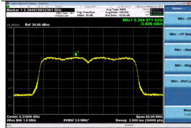
802.11ax40 | Channel 62 | MCS11
