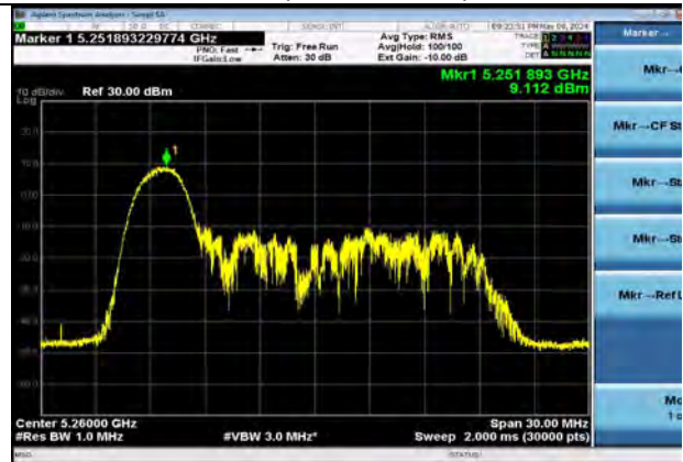
802.11ax20 | Channel 52 | MCS0 | RU26
