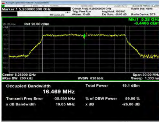
802.11a | Channel 56 | 54 Mbps
