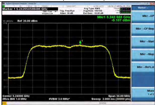
802.11ax20 | Channel 48 | MCS11
