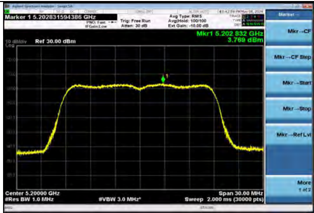
802.11n20 | Channel 40 | MCS7
