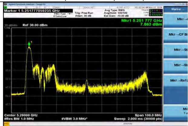
802.11ax80 | Channel 58 | MCS0 | RU26
