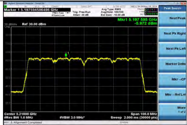
802.11ac80 | Channel 42 | MCS9
