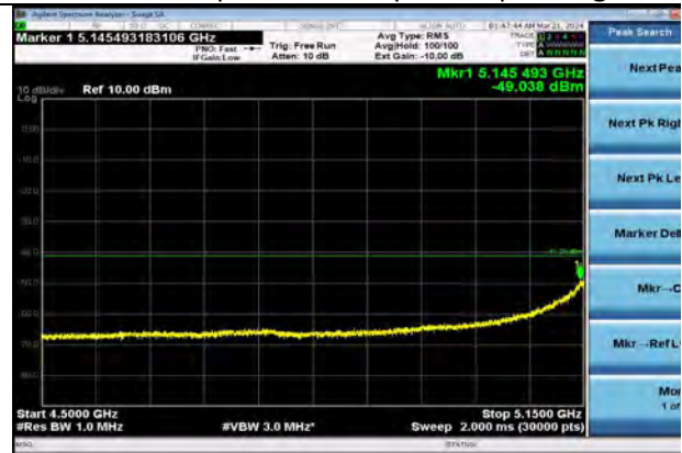
802.11ac40 | Channel 38 | MCS0 | Average
