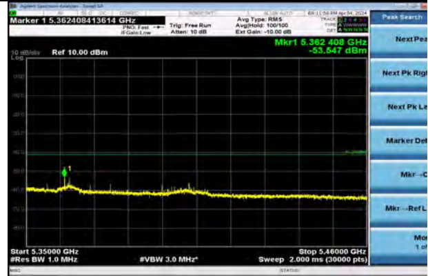
802.11ax20 | Channel 64 | MCS0 | RU52 | Average
