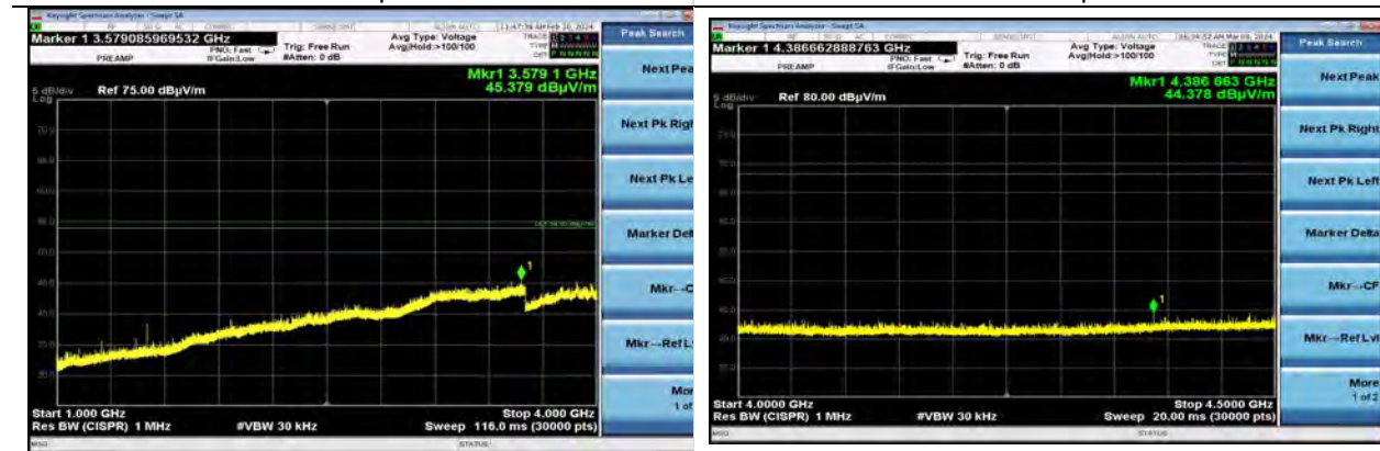
802.11a | Channel 36 | 6 Mbps 1000-4000 MHz | Horizontal
