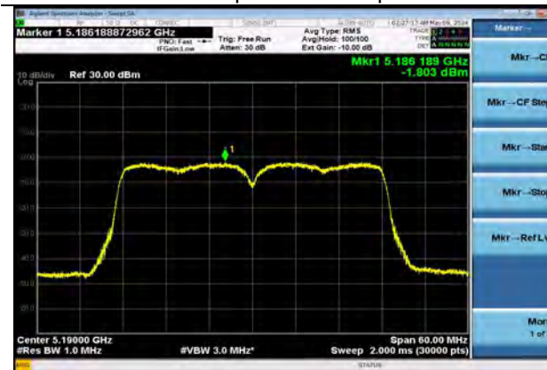
802.11n40 | Channel 38 | MCS7
