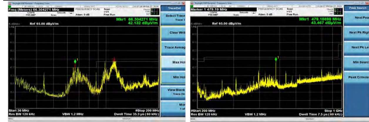
802.11a | Channel 36 | 6 Mbps | Y Plane 30-200 MHz | Vertical
