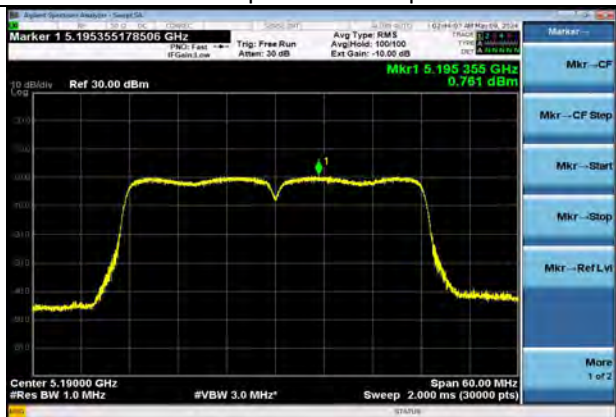
802.11ac40 | Channel 38 | MCS0
