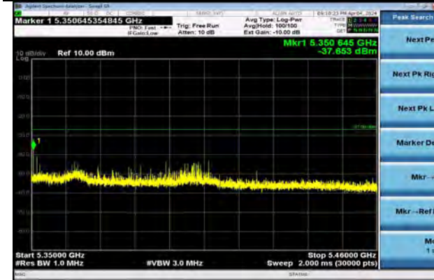
802.11ax80 | Channel 58 | MCS0 | RU52 | Peak
