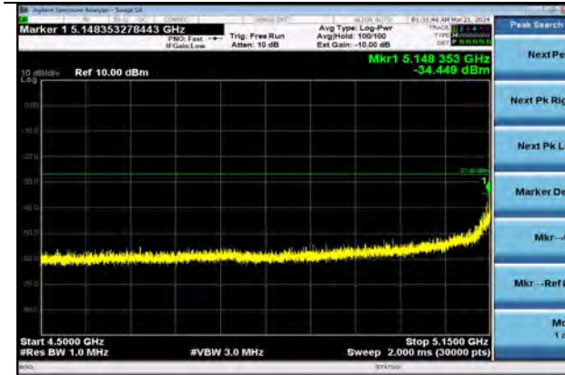
802.11ax20 | Channel 36 | MCS0 | Peak
