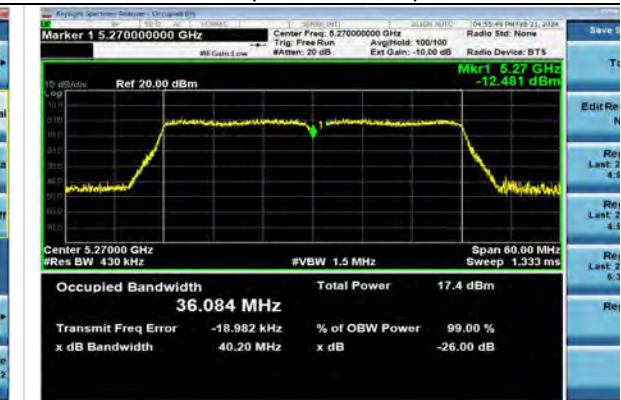
802.11ac40 | Channel 54 | MCS0
