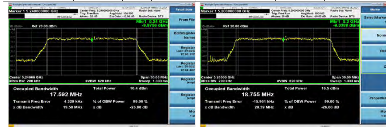
802.11ac20 | Channel 48 | MCS8
