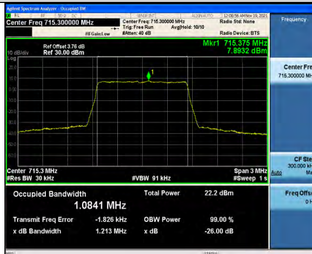
Band12-1.4MHz-QPSK-23173-6RB#0-1.0841
