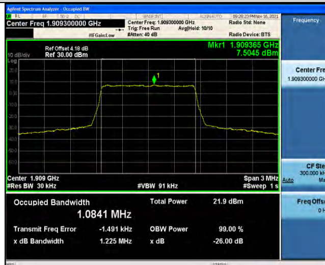
Band2-1.4MHz-QPSK-19193-6RB#0-1.0841
