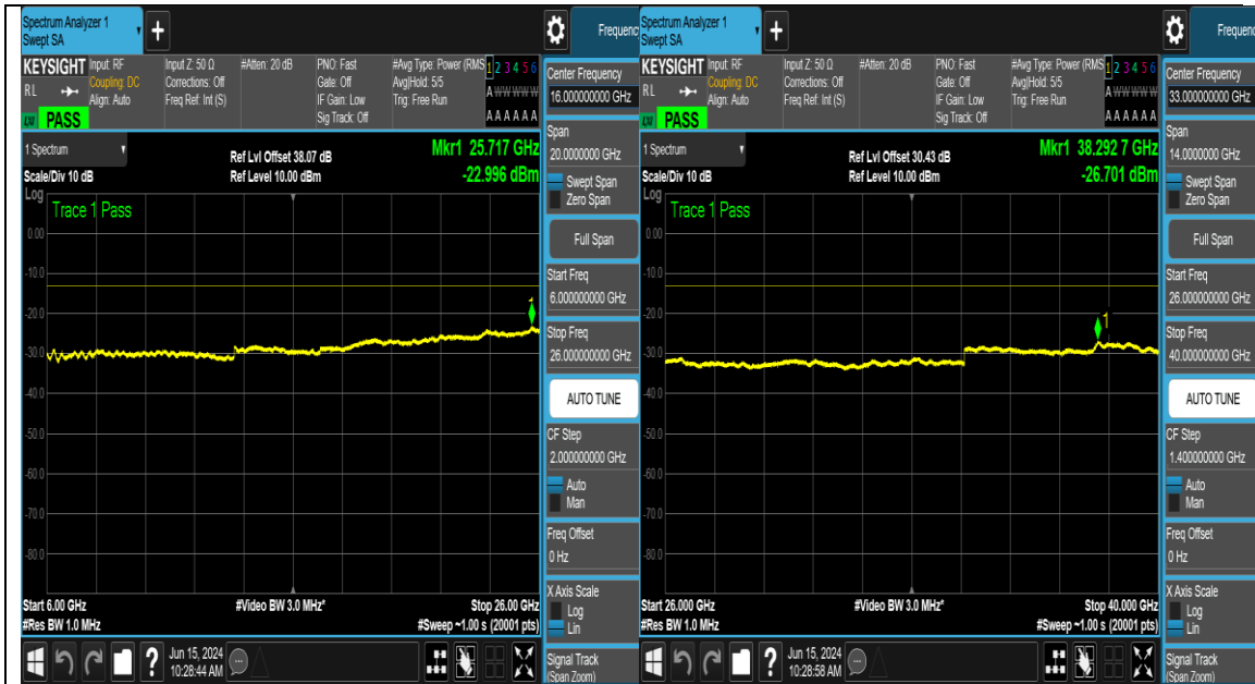
NTNV_N77-3700-3980_PC2_30_80_L_TID16_NS _01_0.009_0.15_#1
