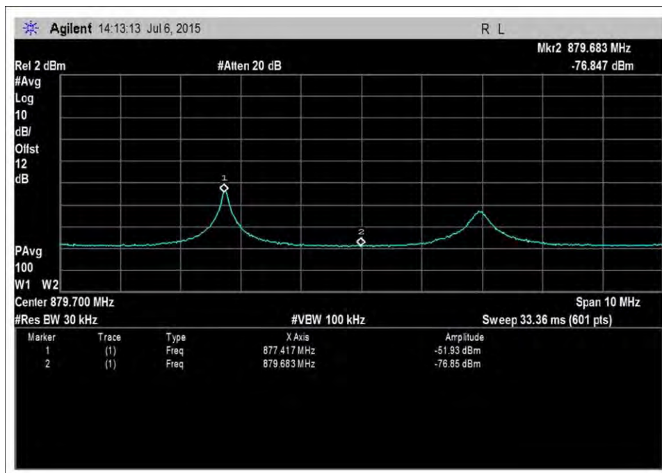
DL_869-894MHz-AWGNL+1
