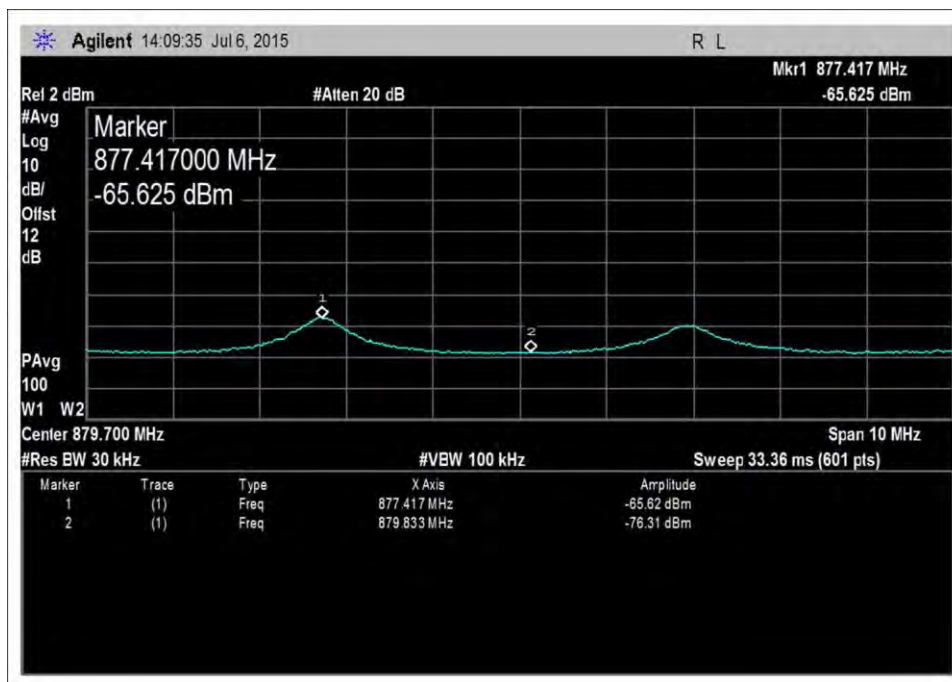
DL_869-894MHz-AWGNL+3
