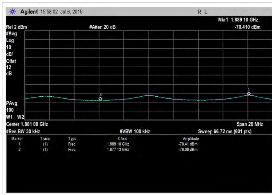
UL_1850-1915MHz-AWGNL+3
