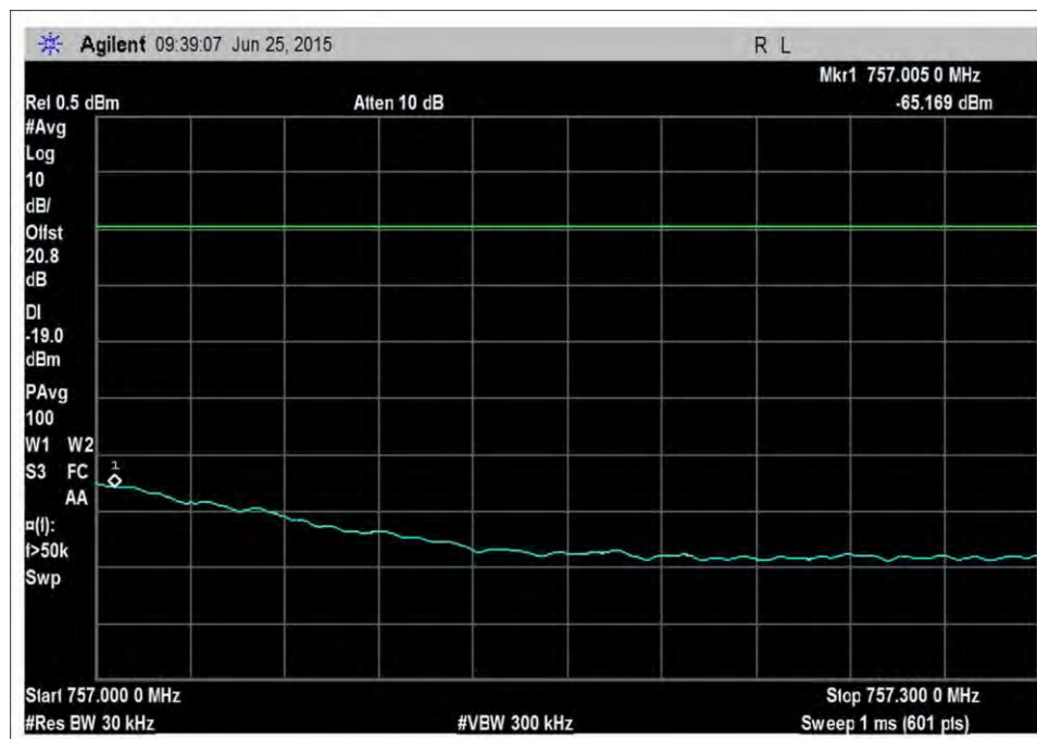
DL_746-757MHz_H_Max
