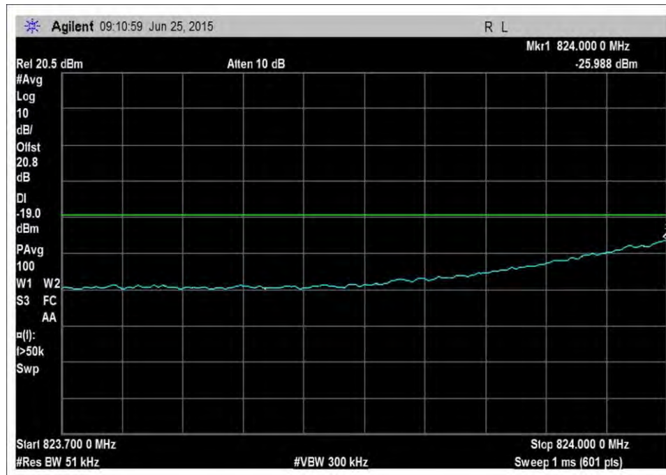
UL_824-849MHz_L_PreAGC
