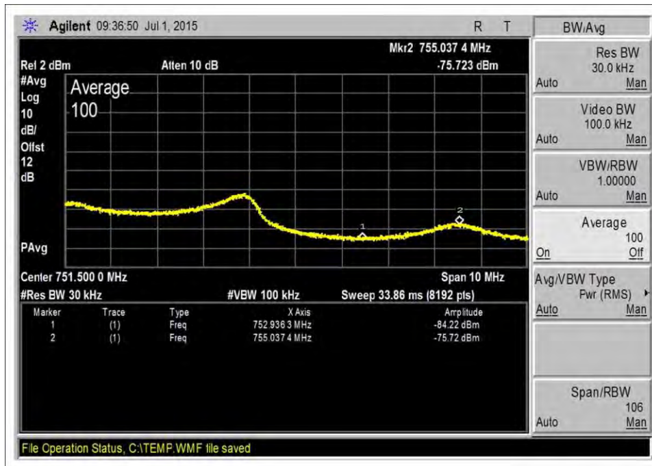
DL_746-757MHz-AWGNL+5
