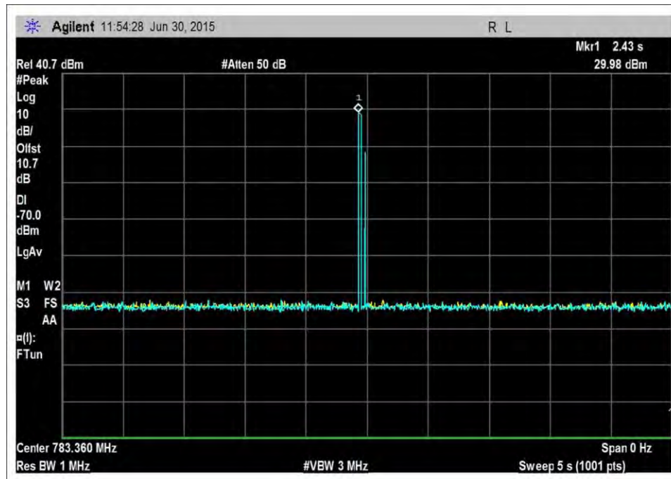
UL_776-787MHz-Pk
