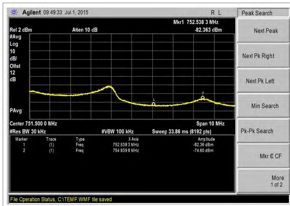
DL_746-757MHz-AWGNL+2
