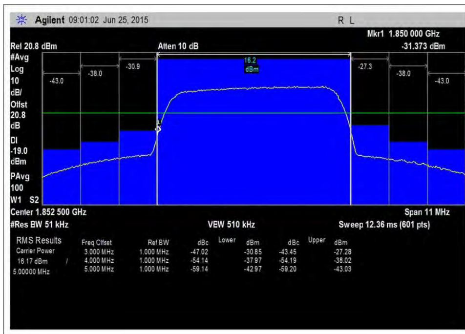
UL_1850-1915MHz_L_PreAGC
