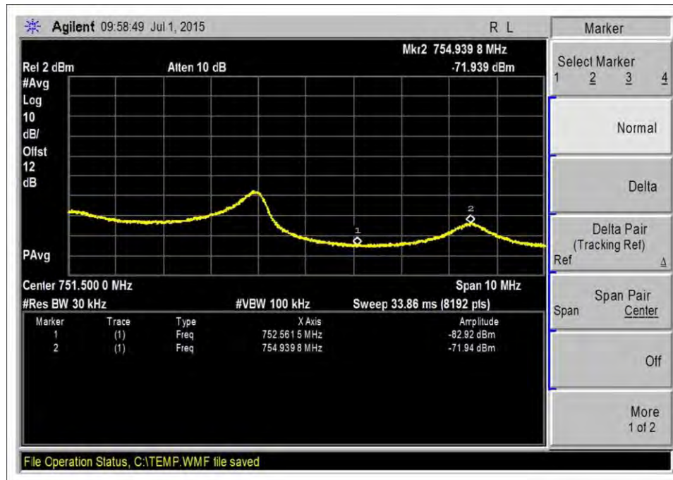
DL_746-757MHz-AWGNL+1
