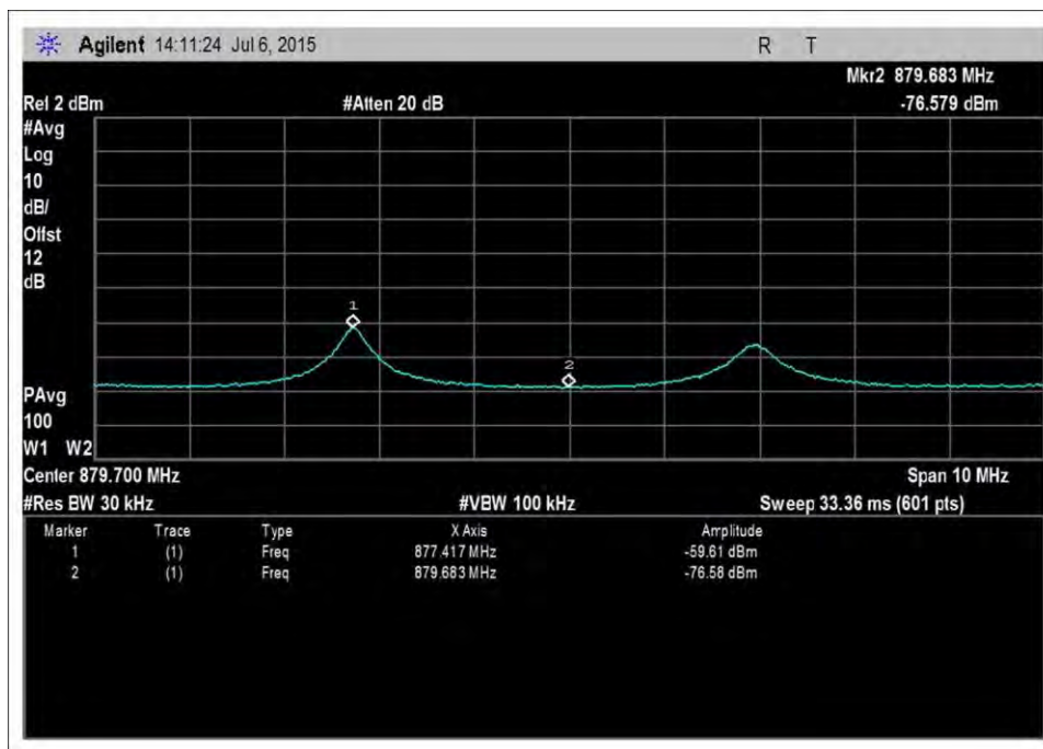
DL_869-894MHz-AWGNL+2
