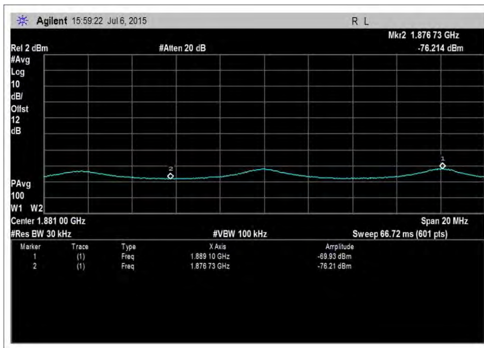
UL_1850-1915MHz-AWGNL+2
