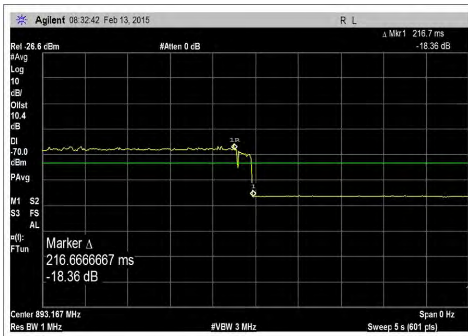
DL_869-894MHz_a-g_timing
