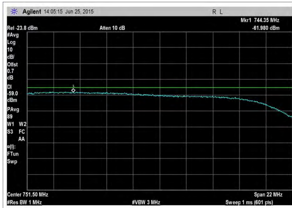
DL_746-757MHz_a-g_Noise_50
