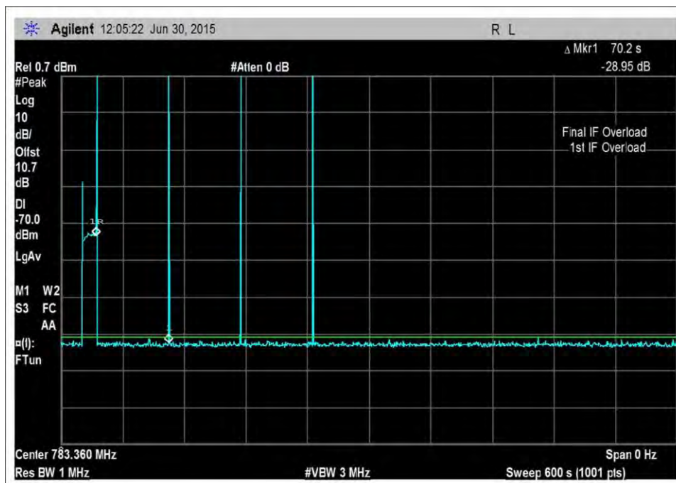
UL_776-787MHz-600sec
