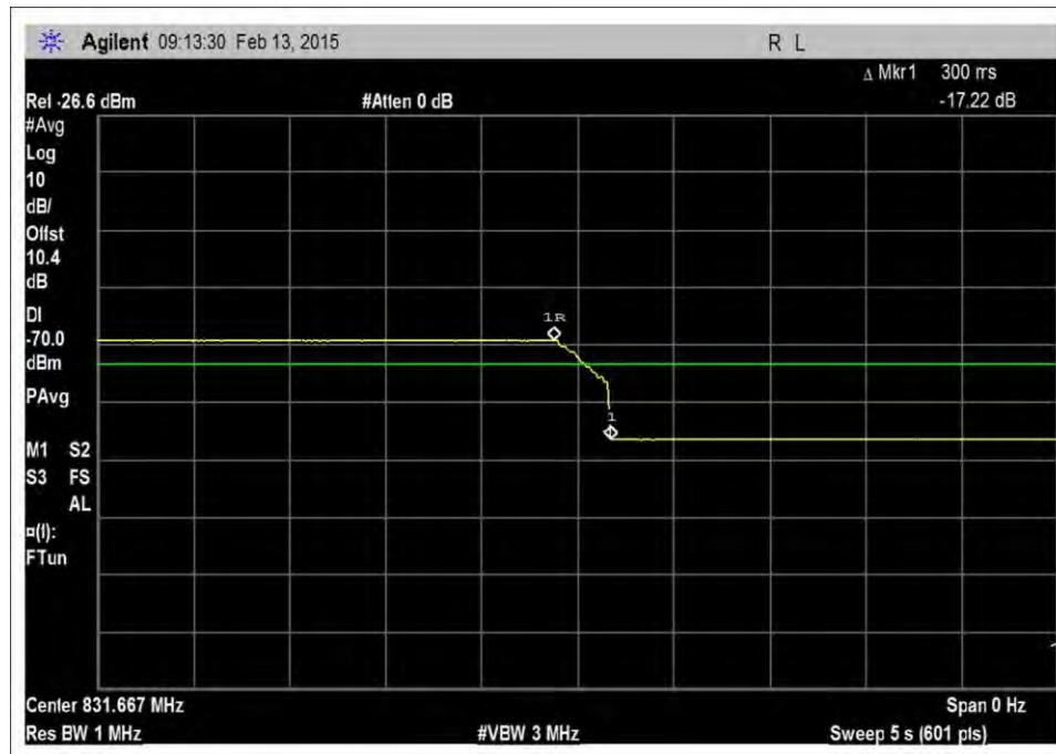
UL_824-849MHz_a-g_timing
