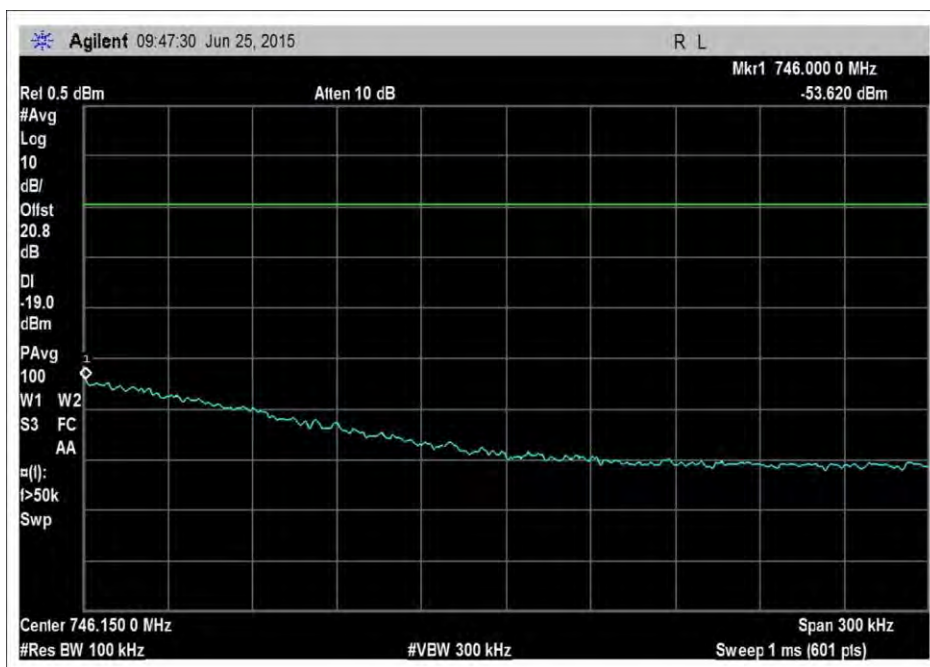
DL_728-746MHz_H_PreAGC
