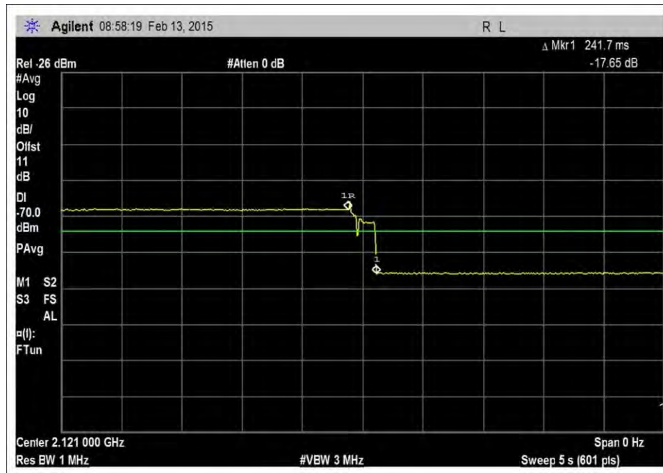
DL_3110-2155MHz_a-g_timing
