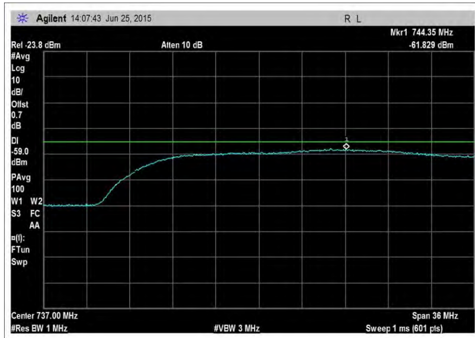
DL_728-746MHz_a-g_Noise_50
