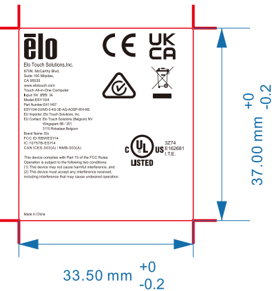
ESY1014,AOSP SAFETY LABEL Artwork for Label Manufacture-White SCALE 1:1 OUTLINE
