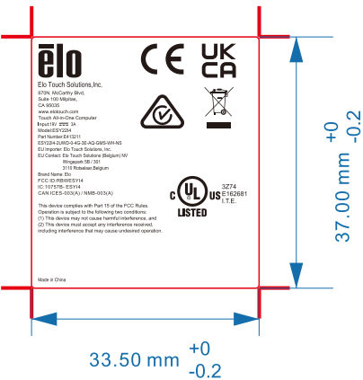
ESY2214,GMS SAFETY LABEL Artwork for Label Manufacture-White SCALE 1:1 OUTLINE
