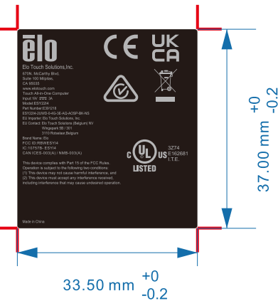
ESY2214,AOSP SAFETY LABEL Artwork for Label Manufacture-Black SCALE 1:1 OUTLINE
