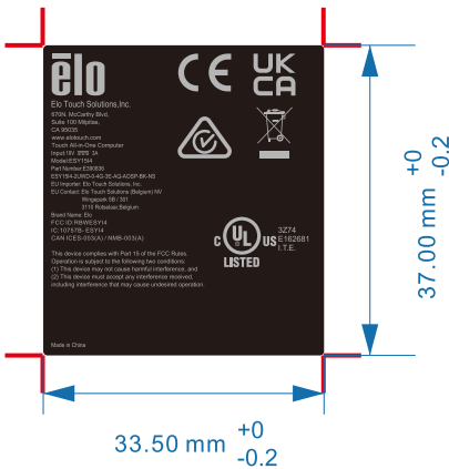
ESY1514,AOSP SAFETY LABEL Artwork for Label Manufacture-Black SCALE 1:1 OUTLINE
