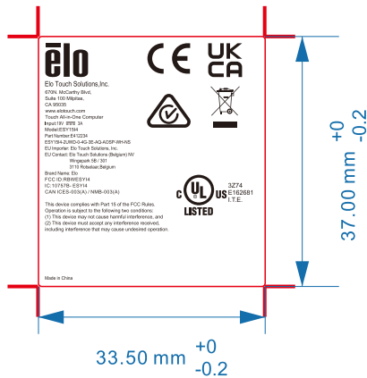
ESY1514,AOSP SAFETY LABEL Artwork for Label Manufacture-White SCALE 1:1 OUTLINE
