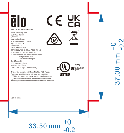
ESY2214,AOSP SAFETY LABEL Artwork for Label Manufacture-White SCALE 1:1 OUTLINE
