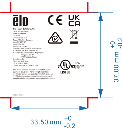
ESY1514,GMS SAFETY LABEL Artwork for Label Manufacture-White SCALE 1:1 OUTLINE
