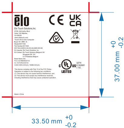
ESY1014,GMS SAFETY LABEL Artwork for Label Manufacture-White SCALE 1:1 OUTLINE
