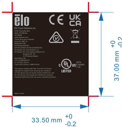
ESY1514,GMS SAFETY LABEL Artwork for Label Manufacture-Black SCALE 1:1 OUTLINE
