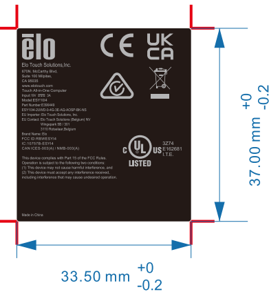
ESY1014,AOSP SAFETY LABEL Artwork for Label Manufacture-Black SCALE 1:1 OUTLINE
