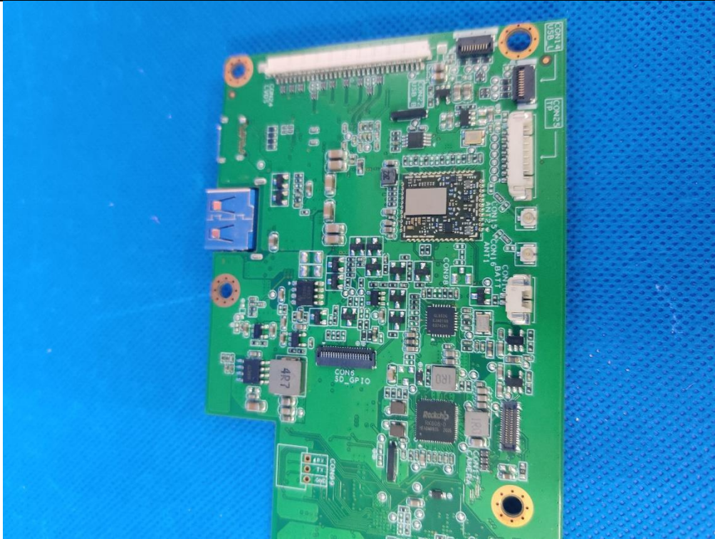
(15) EUT Photo(Model ESY22I4)
