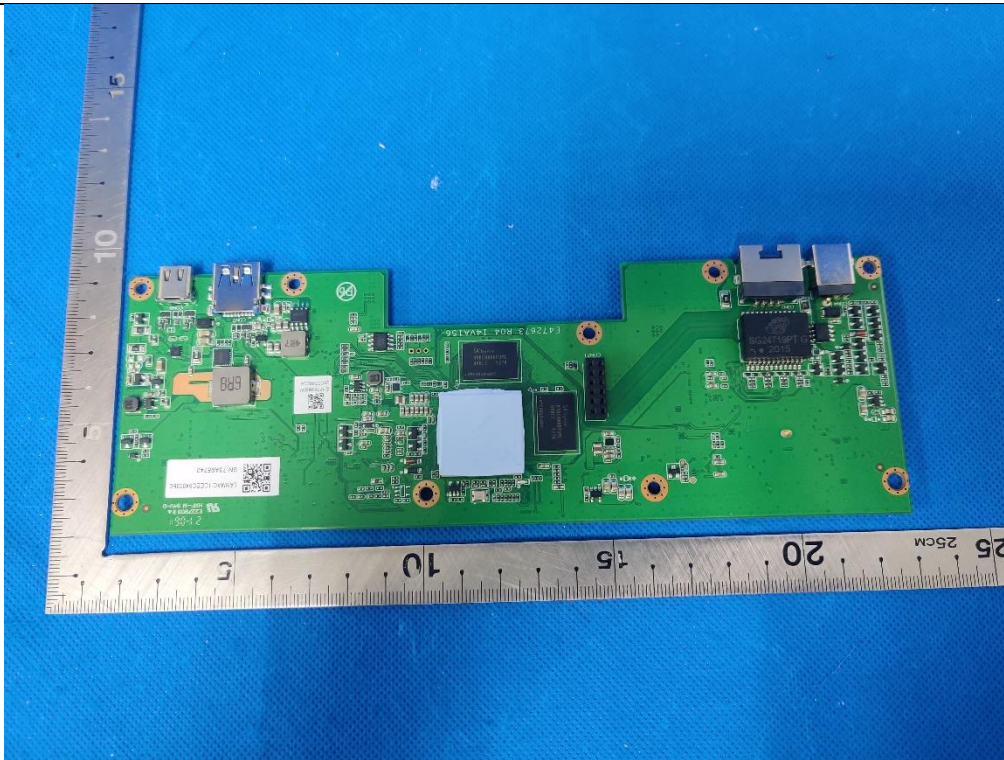
(8) EUT Photo(Model ESY1514)
