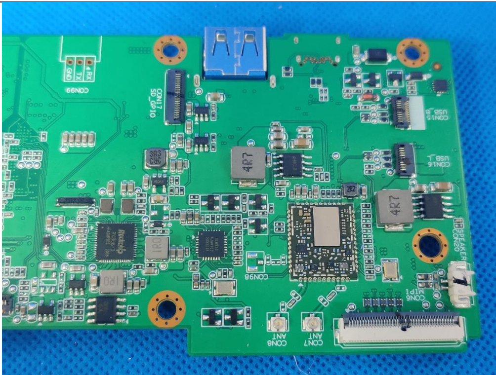
(6) EUT Photo(Model ESY15I4)
