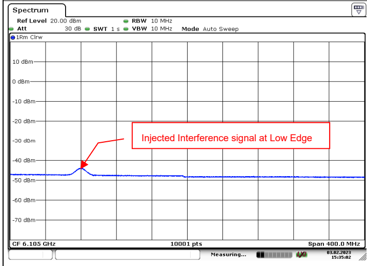
802.11be (EHT320) / CH31 (Low Edge)
