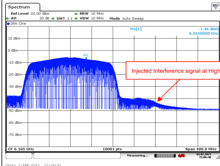
802.11be (EHT320) / CH31 (High Edge)
