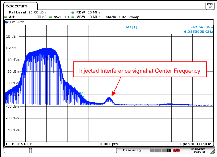
802.11be (EHT320) / CH31 (Middle)
