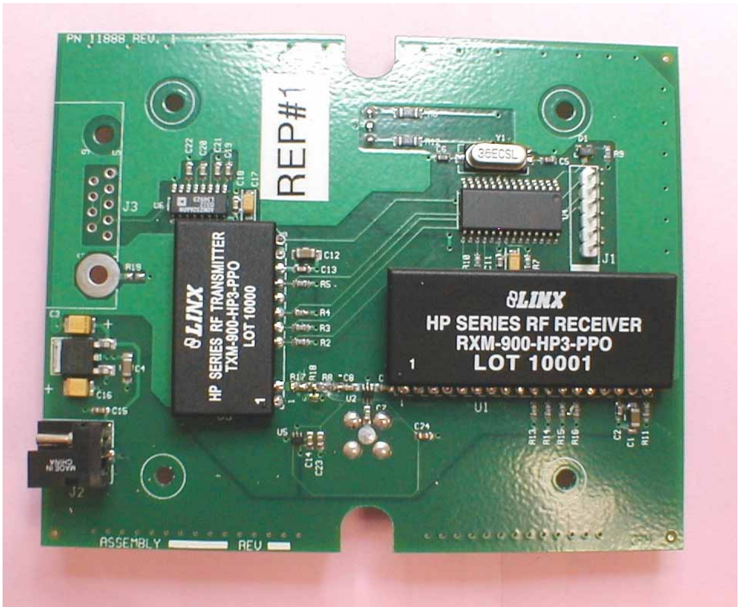
Top View of PCB
